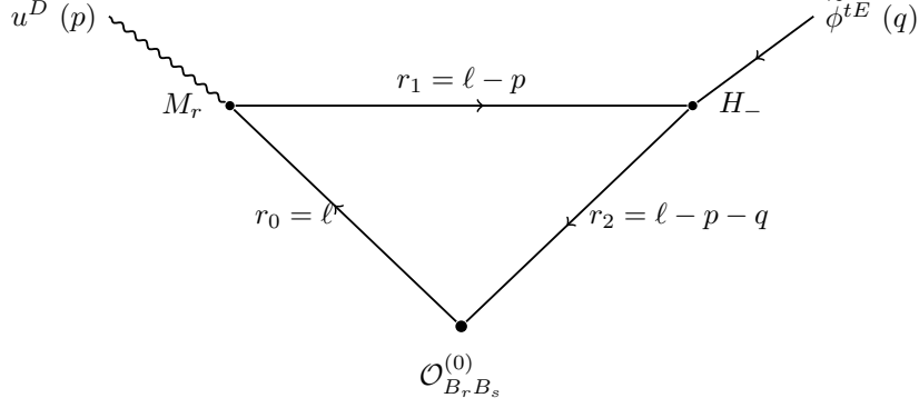
Figure 7: The ordered triangle of route 002 for the (\beta_r, \beta_s) channel, r \neq s , drawn in the unit normalization (4.182). The composite insertion \mathcal{O}_{B_r B_s}^{(0)} (filled node) attaches to the matter vertex M_r and to the superpotential vertex H_- ; the three internal lines are chiral–antichiral matter propagators with the displayed routing; the external legs are the unit prepotential u^D (wavy) and the antichiral field \tilde{\phi}^{tE} , converted to the letters \partial c and \gamma^t by the external map (4.195). Route 003 is the independently oriented partner with reversed ports and the rebase (4.188).
