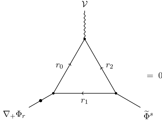
Figure 8: The representative ordinary matter-triangle parent of the (\beta_r, \gamma^s) family. The three edges are matter propagators with edge momenta r_0, r_1, r_2 , denominators D_i = r_{i,d}^2 ; the two ordered sources are the marked insertion \nabla_+ \Phi_r (filled node) and the antichiral leg \tilde{\Phi}^s ; the external field-strength letters enter through the preimages \tilde{\mathcal{W}}_{\dot{\alpha}}^{(1)} = -\frac{1}{8} \mathcal{D}^2 \bar{\mathcal{D}}_{\dot{\alpha}} \nu on the vector leg. Every ordinary parent of the family vanishes on the physical output word \langle \partial c, \partial c \rangle , as displayed; the kernels themselves are nonzero (Remark 4.36). The anomaly is instead the regulated coincident Euler Jacobian of the kinetic occurrence (4.238).
