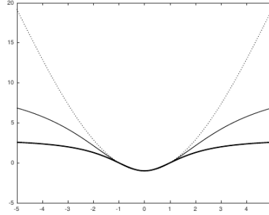
Figure 10.1: Beta-t-EGARCH: Response of u_t to a standardised observation y_t for \nu = 3, 10, 100 ( \nu = 100 is parabola, \nu = 3 almost flat)
