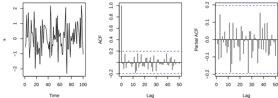
Gaussian WN realization
