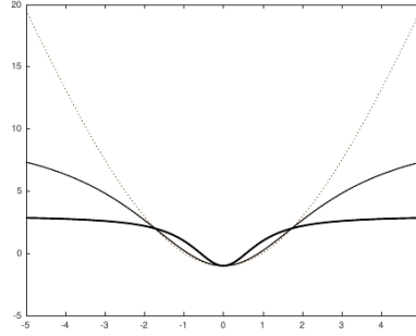
Figure 10.2: Beta-t-GARCH: Response of u_t to a standardised observation y_t for \nu = 3, 10, 100 ( \nu = 100 is parabola, \nu = 3 almost flat)
