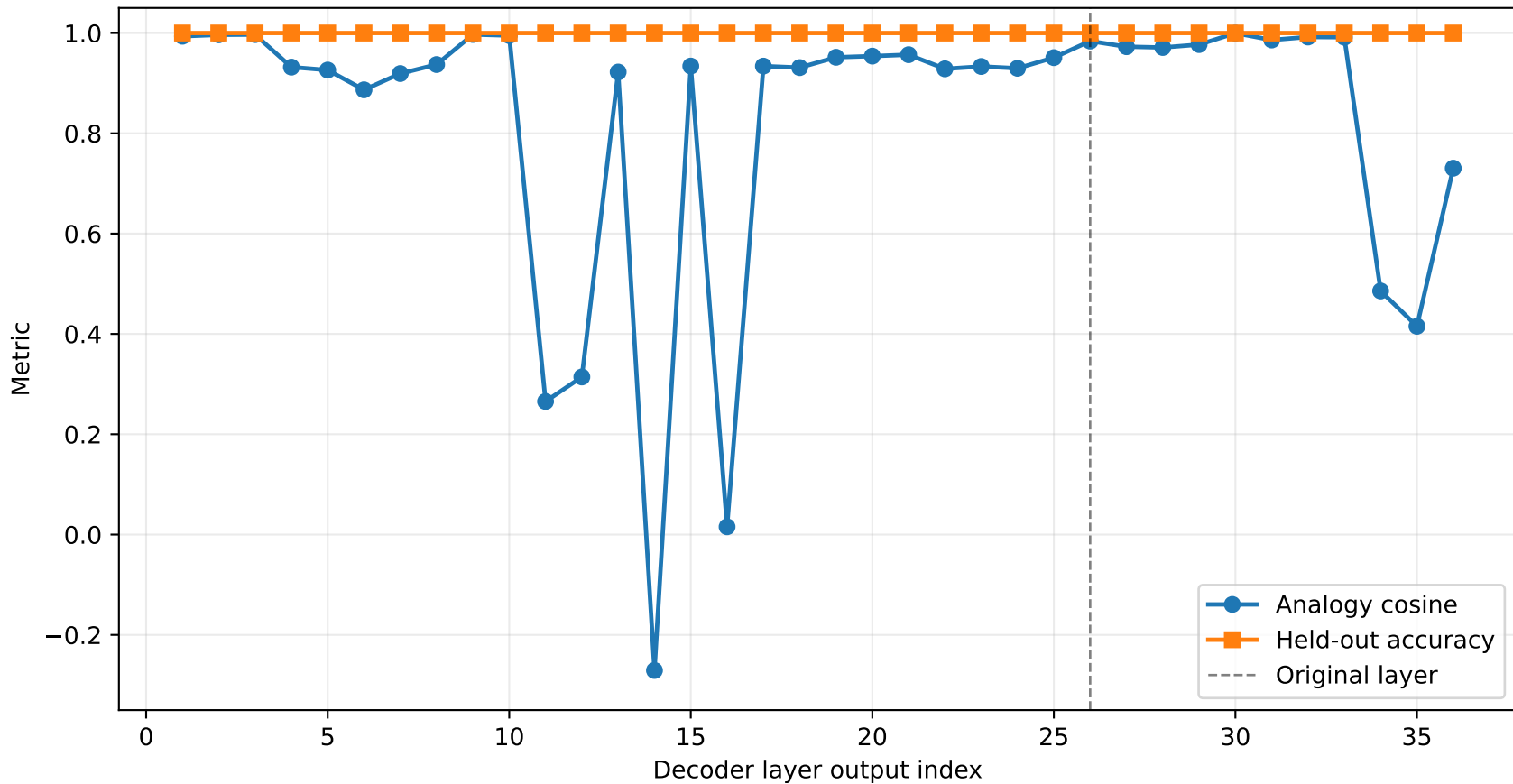
Classification-only layer sweep
