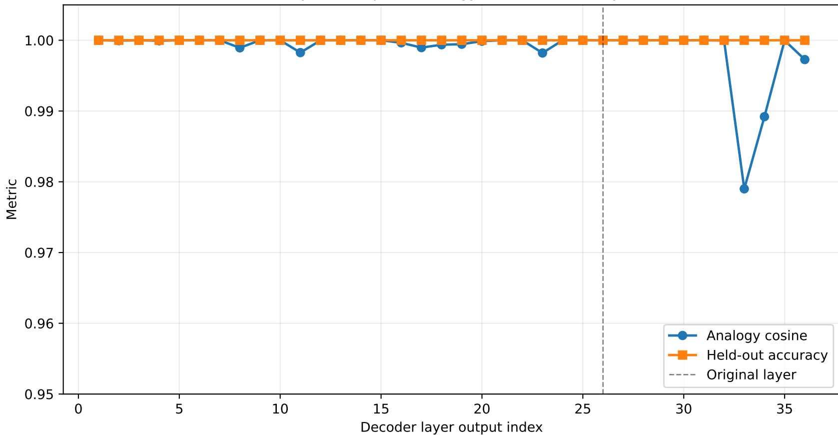
Layer sweep for analogy-codec readability
