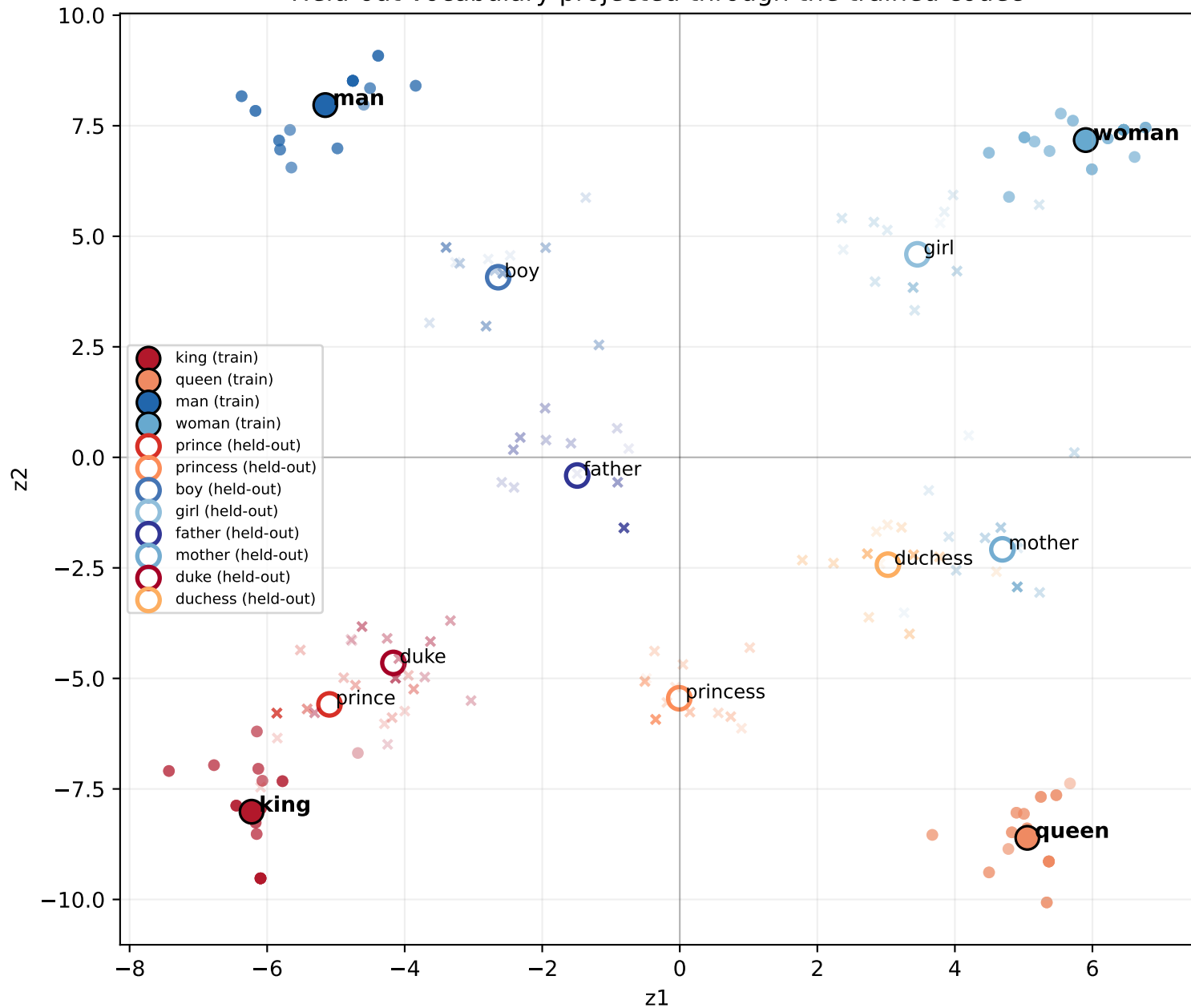
Held-out vocabulary projected through the trained codec
