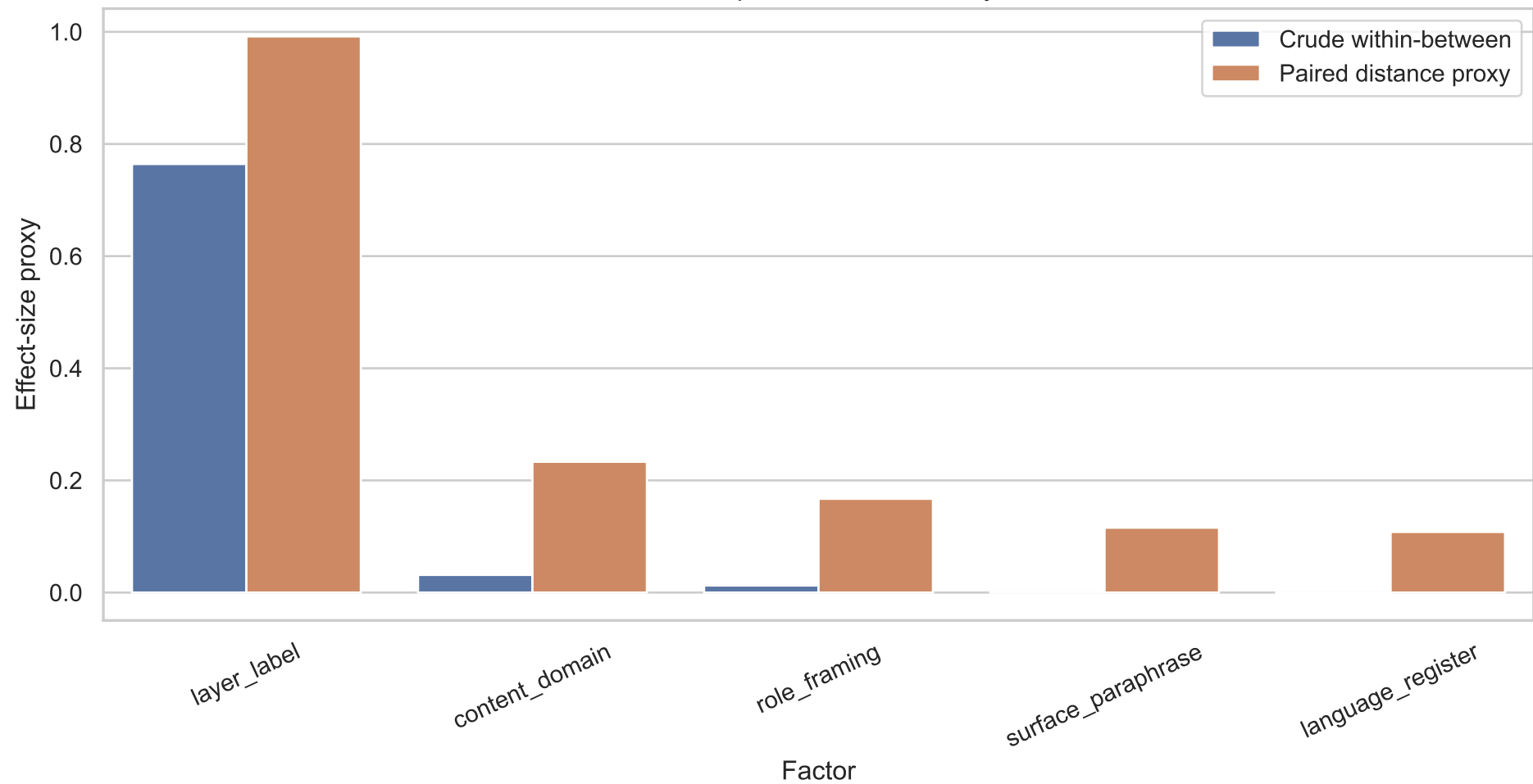
Crude feature-pattern disturbance by factor
