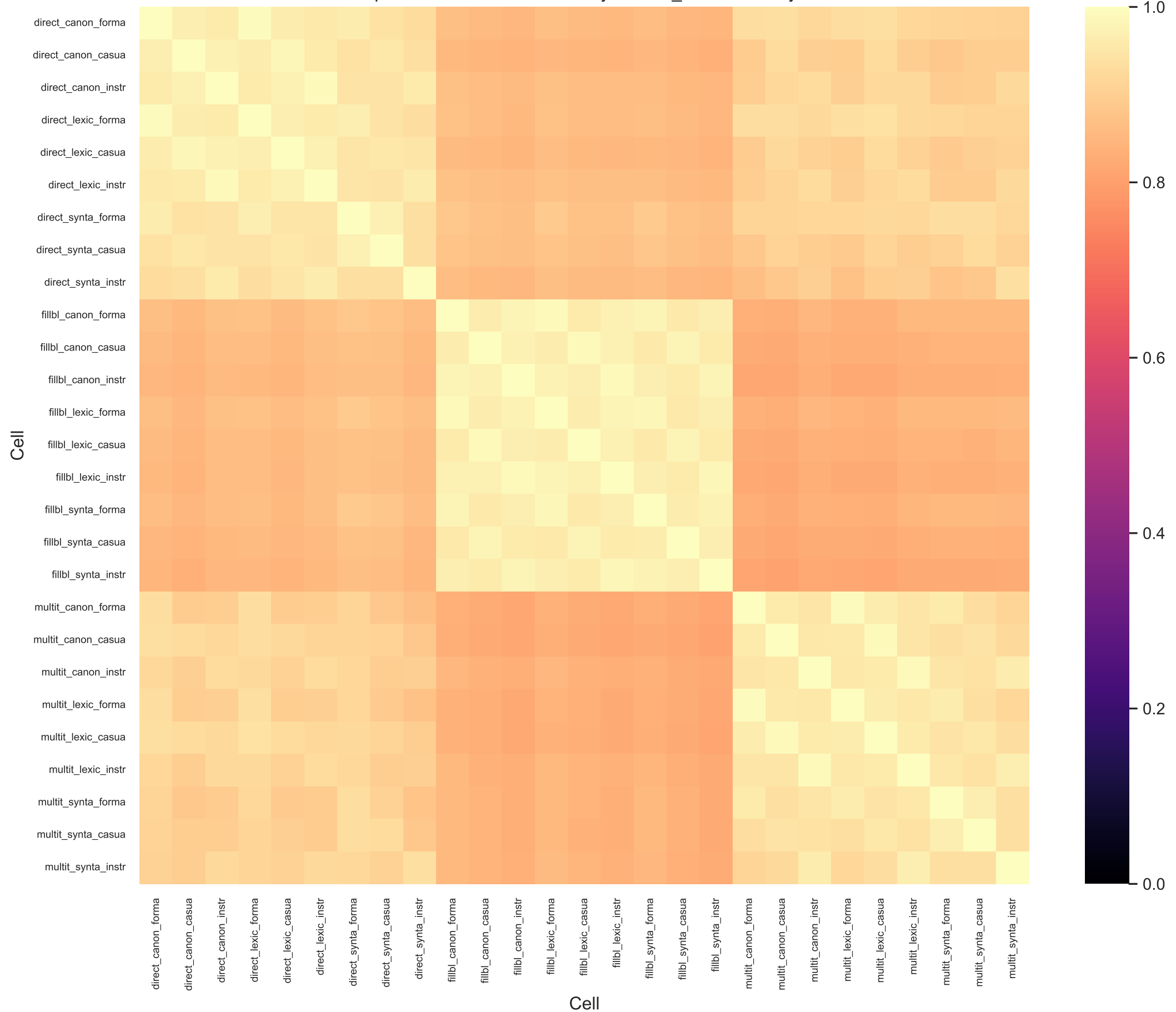
Full-spectrum SAE cosine similarity: factual_recall / fr1 / layer 12
