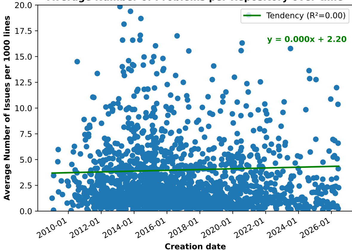
Average Number of Problems per Repository over time
