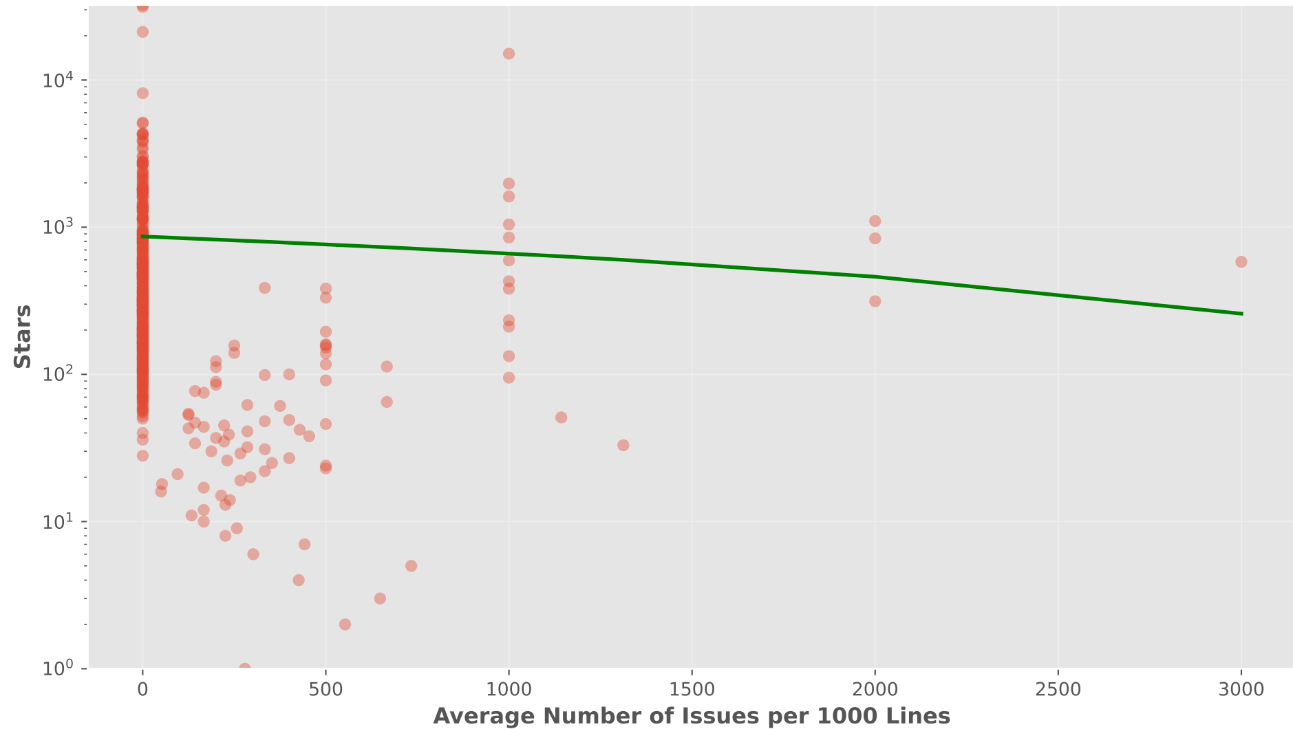
Repository Popularity vs Issue Density (per 1000 Lines)
