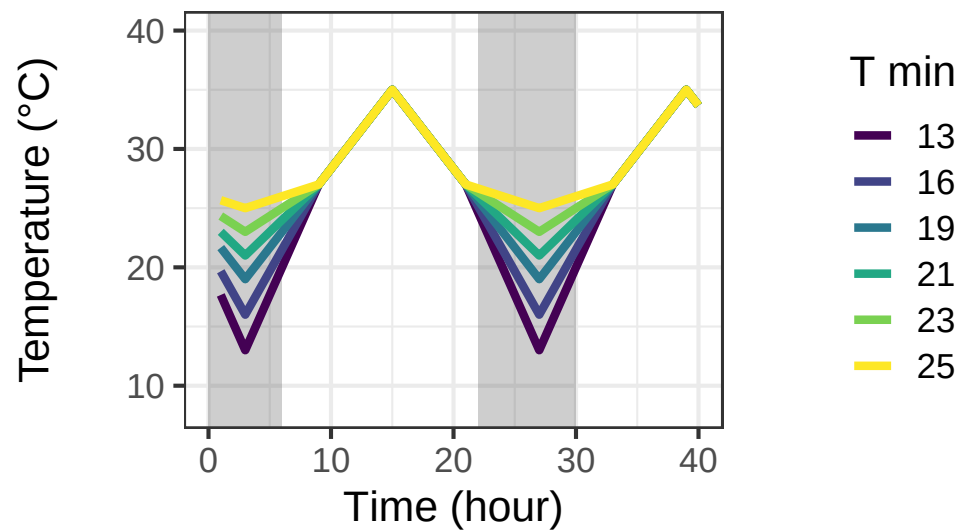
C) expt 3. vary fluctuations
