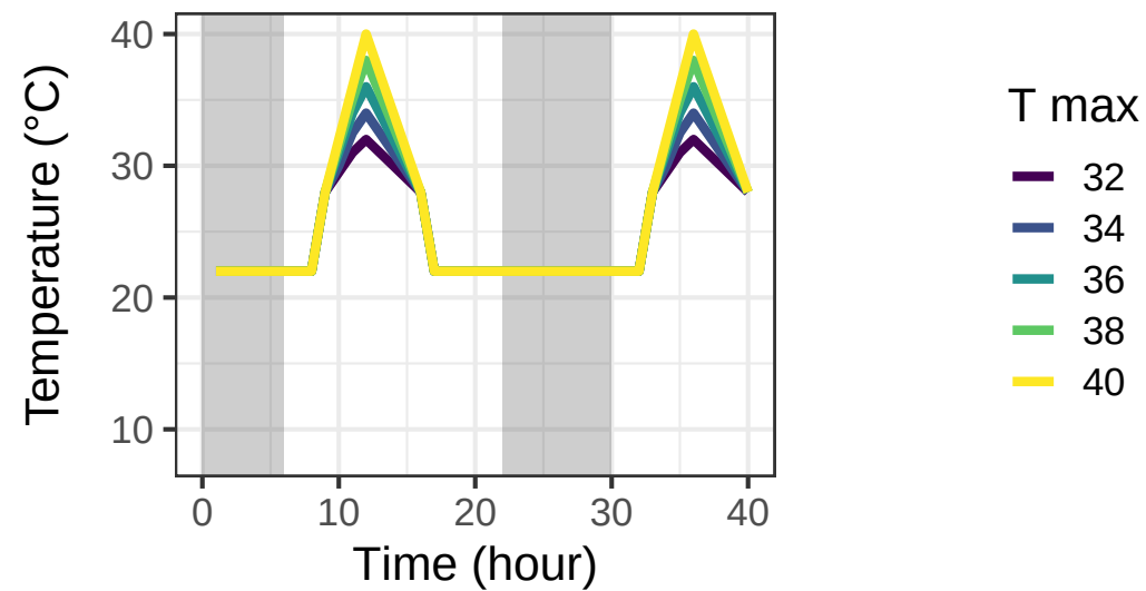
D) expt 4. vary mean and fluctuations
