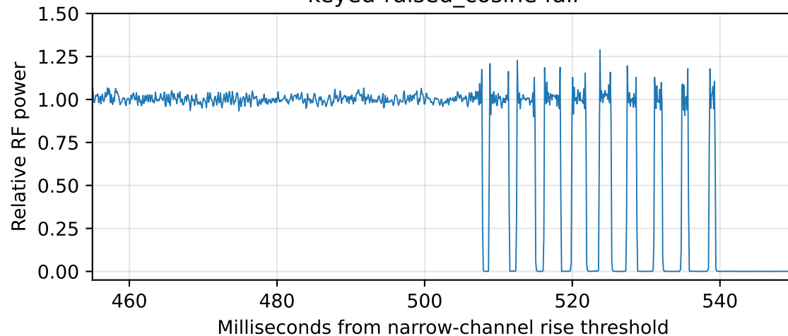
keyed-raised_cosine fall
