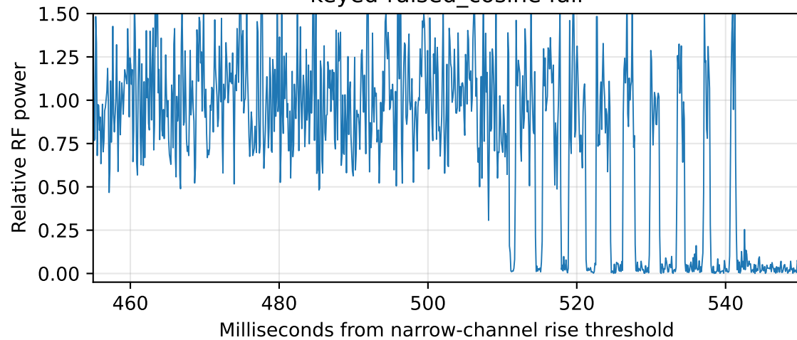
keyed-raised_cosine fall
