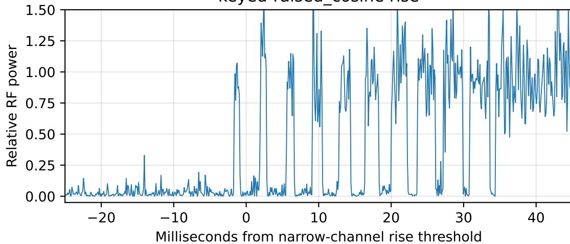
keyed-raised_cosine rise
