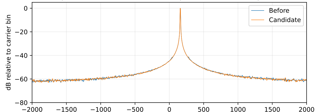
Spectrum: carrier interiors / complete modulation sequence
