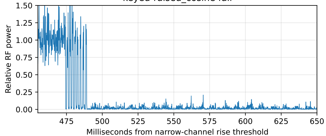
keyed-raised_cosine fall
