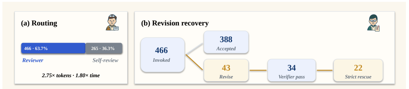
Figure 4. Adaptive Reviewer routing and revision recovery. Panel (a) shows that 466 of 731 tasks invoke an independent Reviewer, while 265 use Engineer self-review; routed tasks consume 2.75\times the solve input Tokens and 1.80\times the active time on average. Panel (b) follows the routed workload: 388 tasks are accepted on first review, 43 receive a revision request, 34 of those later pass the official verifier, and 22 complete the strict review-loop rescue. Routing is task-dependent, so the cost contrast is descriptive rather than a randomized causal estimate.
