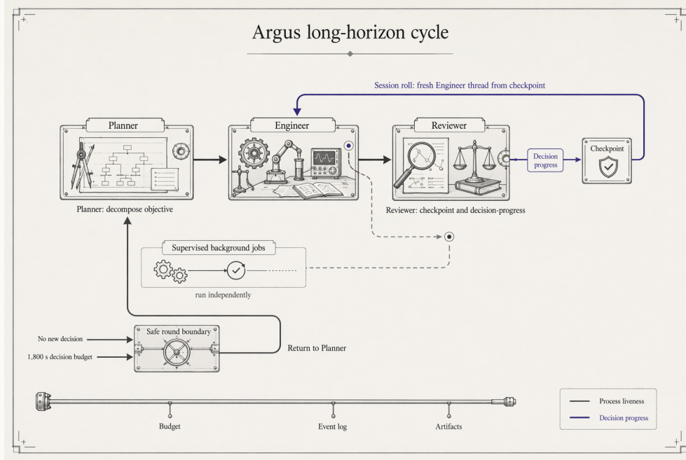
Figure 2: System schematic (not a measured performance plot) of the Argus long-horizon reliability cycle: Planner, Engineer, and Reviewer run one continuous loop; the Reviewer emits a single bounded checkpoint and a decision-progress class that reseeds a fresh Engineer thread; supervised background jobs run independently alongside the loop; and a safe round boundary returns a stalled or budget-exhausted mission to the Planner, all on top of a persistent budget, event-log, and artifact rail.
