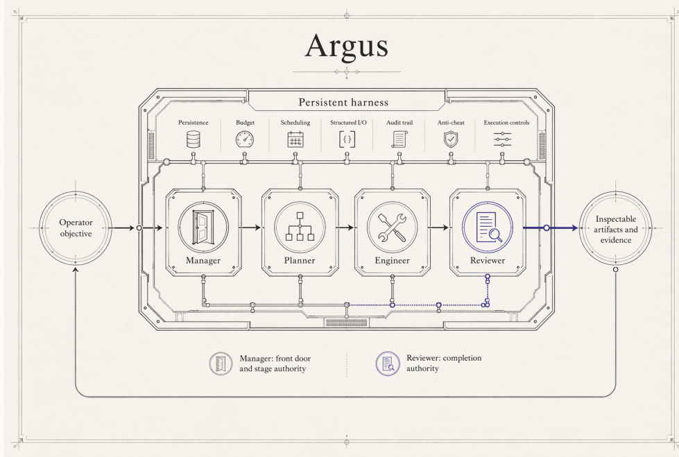
Figure 1: System schematic (not a measured performance plot) of the Argus architecture: an operator objective enters a persistent, domain-agnostic harness; the Manager, Planner, Engineer, and Reviewer sit inside it as the four roles that make every research judgment; and inspectable artifacts and evidence exit back to the operator.
