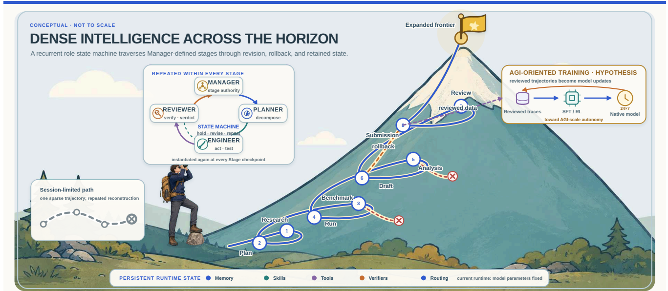
Figure 2. Conceptual view of Dense Intelligence across the effective task horizon. The four roles form a recurrent state machine instantiated inside every stage: Manager owns stage transitions, Planner decomposes work, Engineer acts and tests, and Reviewer returns a verdict that can trigger revision. The research vertical is shown with eight stages—research, plan, benchmark, run, analysis, draft, review, and submission. A binocular-equipped researcher stands on the connected foreground ridge and looks toward the golden summit flag. The sand-backed blue route follows mountain switchbacks, rising overall while including local descents; the orange dashed arrow is a rollback, and red crosses are rejected branches. The purple flow sends reviewed trajectories to a future SFT/RL flywheel whose target is native long-horizon behavior. That parameter-training panel is a research hypothesis; the current runtime keeps model parameters fixed. Geometry and height are schematic rather than empirical scales.
