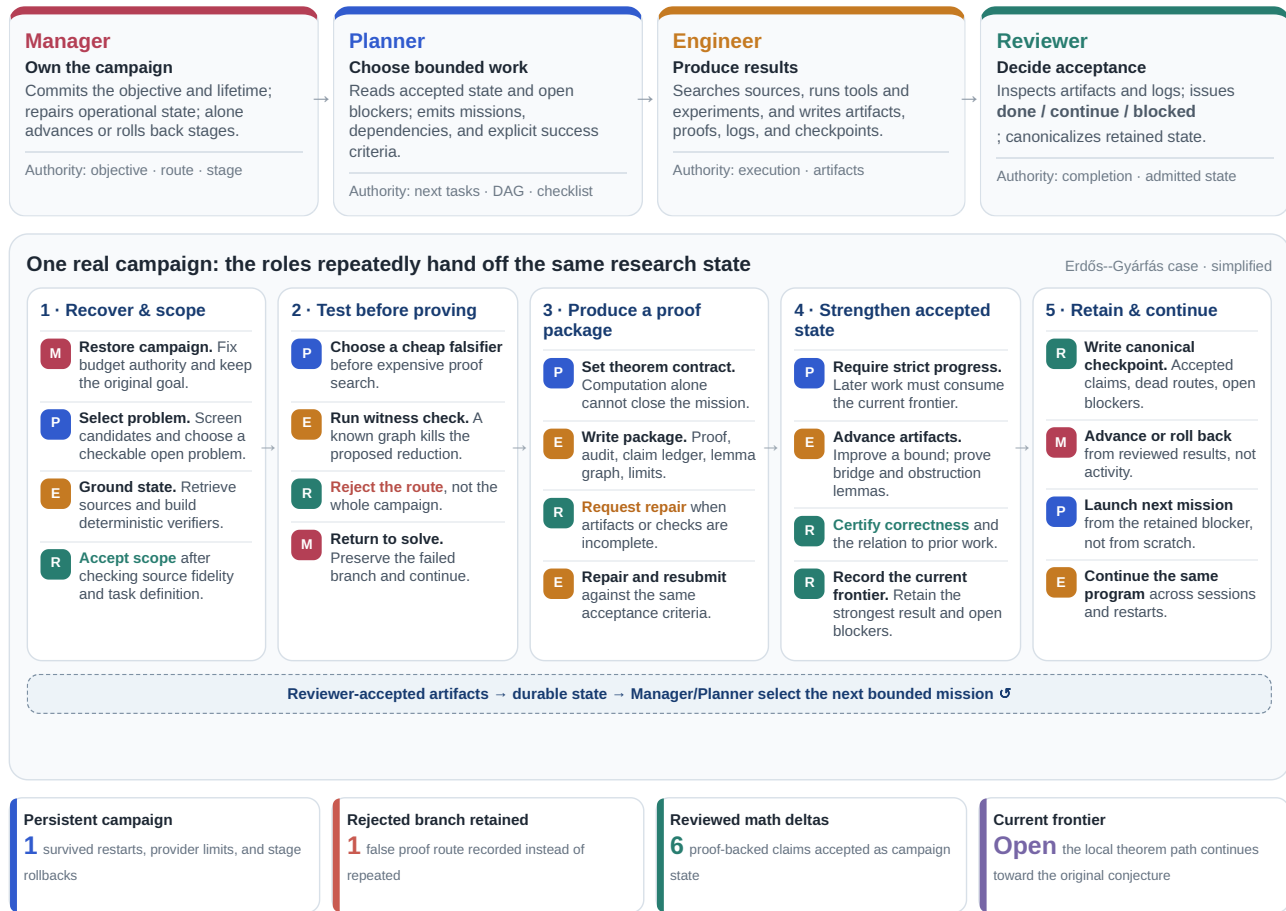
Figure 5. Role-resolved execution of one vertical research campaign. Panel A states the four authorities. Panel B follows the same campaign through recovery, scope, route testing, proof production, revision, strengthening, and retained state. Bottom cards summarize the mathematical outputs accumulated by the campaign.
