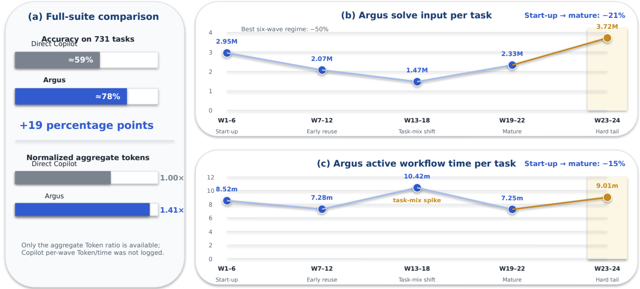
Figure 3. Analysis of the SWE-Bench Pro result. The left panel repeats the full-suite comparison; the right panels aggregate Argus Token and active time over approximately six-Wave windows. The task-mix spike and hard tail are retained. Copilot per-Wave resource traces are unavailable.
