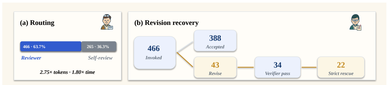
Figure 4. Adaptive Reviewer routing and revision recovery. Panel (a) shows that 466 of 731 tasks invoke an independent Reviewer, while 265 use Engineer the historical self-review route; routed tasks consume 2.75\times the solve input Tokens and 1.80\times the active time on average. Panel (b) follows the routed workload: 388 tasks are accepted on first review, 43 receive a revision request, 34 of those later pass the official verifier, and 22 complete the strict review-loop rescue. Routing is task-dependent, so the cost contrast is descriptive rather than a randomized causal estimate.
