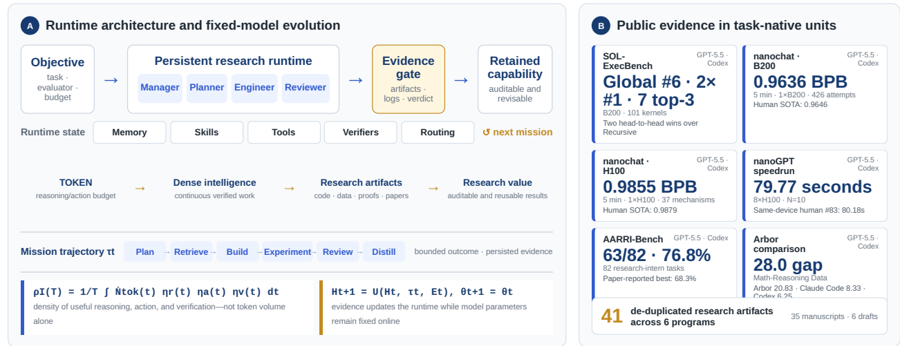
Figure 1. ARGUS at a glance. (A) A dense-intelligence objective enters a role-separated runtime; artifacts and review evidence pass through an evidence gate before updating reusable state around a fixed model. (B) The current public record spans six heterogeneous arenas and 41 research artifacts. Result cards preserve task-native units and identify GPT-5.5 as the agent backbone and Codex as the backend; they are not cross-normalized.
