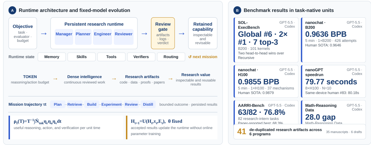
Figure 1. ARGUS at a glance. (A) A dense-intelligence objective enters a role-separated runtime; artifacts and run results pass through a review gate before updating reusable state around a fixed model. (B) The current public record spans six heterogeneous arenas and 41 research artifacts. Result cards preserve task-native units and identify GPT-5.5 as the agent backbone and Codex as the backend; they are not cross-normalized.
