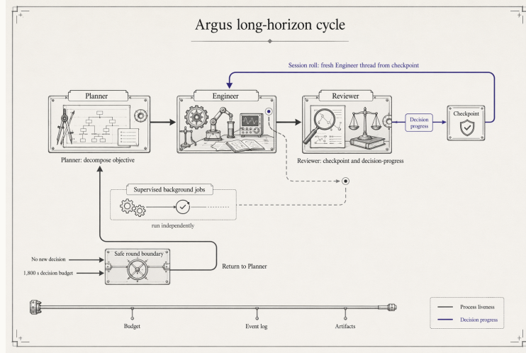
Figure 4. System schematic (not a measured performance plot) of the long-running reliability cycle: Planner, Engineer, and Reviewer run one loop; the Reviewer maintains a bounded curated checkpoint and a decision-progress class that guides the next Engineer round; supervised background jobs run alongside; and a safe round boundary returns a stalled or budget-exhausted mission to the Planner, over a persistent budget, event-log, and artifact rail.
