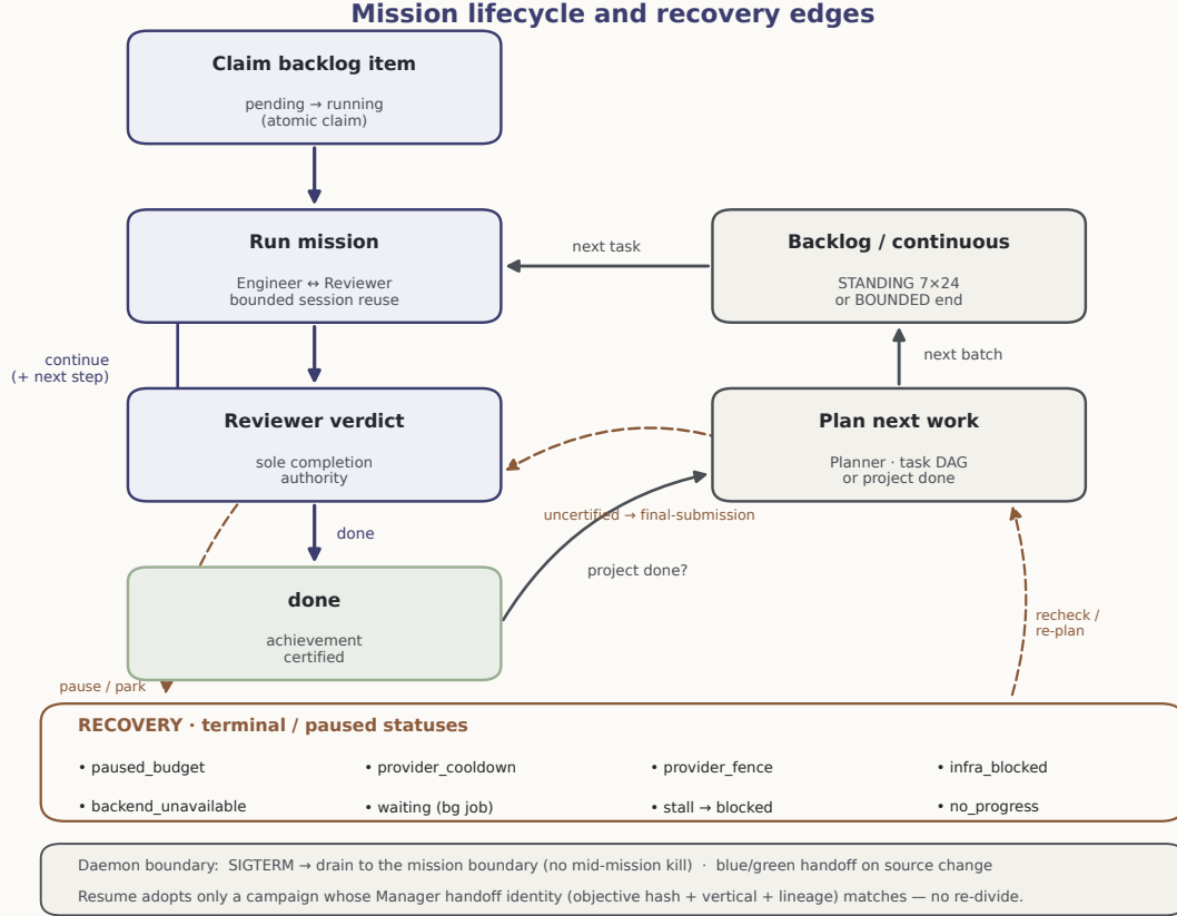
Figure 3. Mission lifecycle and recovery edges. The primary spine (indigo) claims a backlog item, runs an Engineer↔Reviewer mission, and acts on the Reviewer verdict; the plan-next loop (grey) refills the backlog; recovery edges (terracotta) route paused and blocked missions to first-class statuses and back. The daemon boundary governs draining, handoff, and identity-checked resume.
