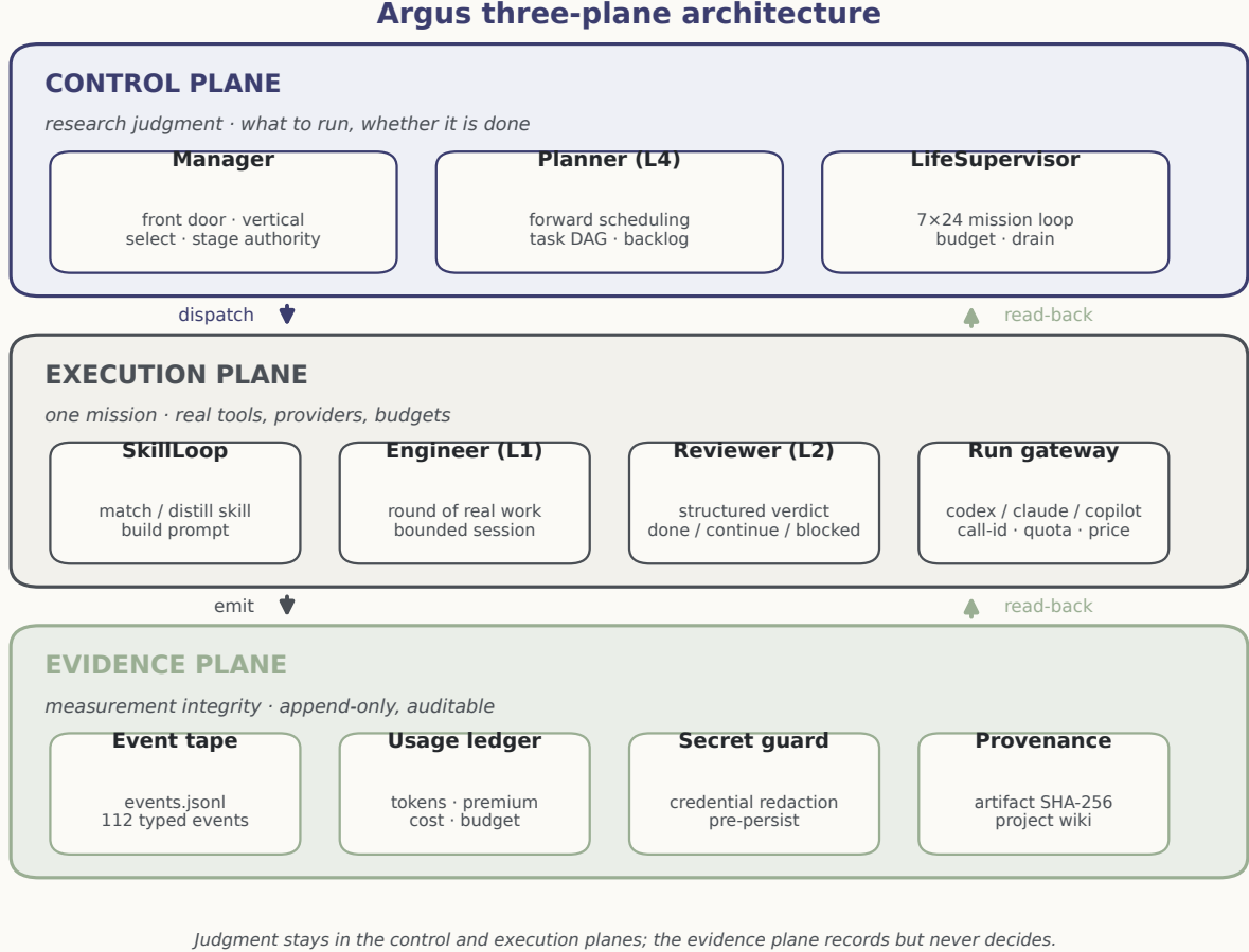
Figure 1. The three-plane architecture. Control-plane roles dispatch work into the execution plane, which emits typed events into the evidence plane; the evidence plane is read back by both other planes but holds no decision authority. Drawn deterministically from the module map (Appendix D).
