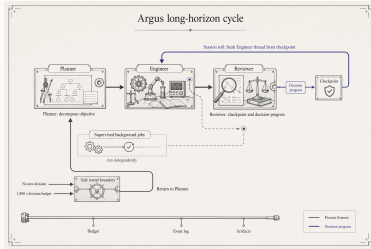
Figure 4. System schematic (not a measured performance plot) of the long-running reliability cycle: Planner, Engineer, and Reviewer run one loop; the Reviewer maintains a bounded shared note and a decision-progress class that guides the next Engineer round; supervised background jobs run alongside; and a safe round boundary returns a stalled or budget-exhausted mission to the Planner, over a persistent budget, event-log, and artifact rail.
