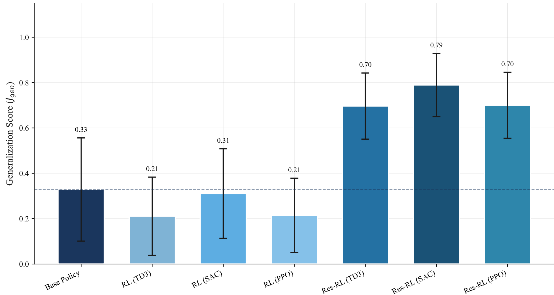
Generalization Performance (OOD Trials 11–20) (Averaged Across All Tasks)
