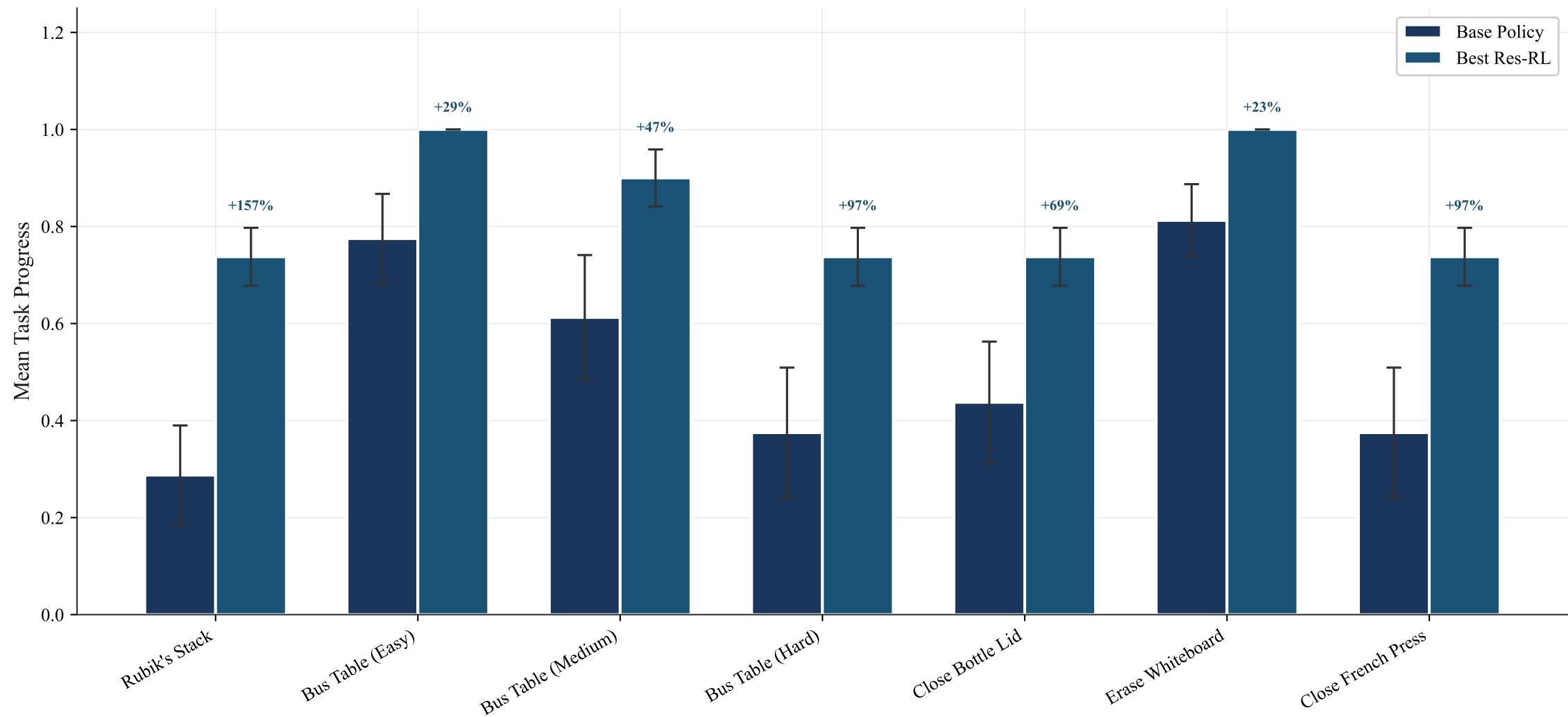
Per-Task Performance: Base Policy vs Best Residual RL
