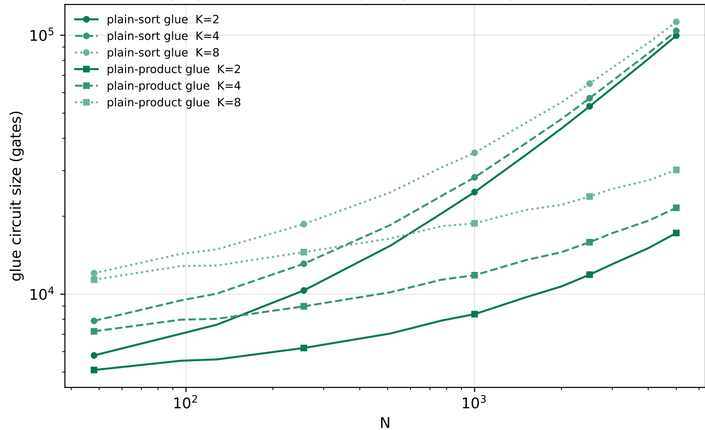
The fingerprint lever — sort glue grows O(N) , product glue O(K)
