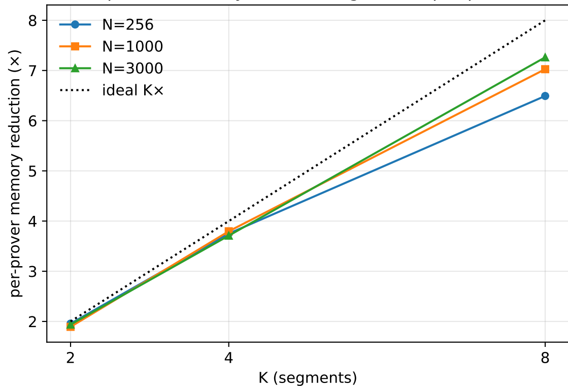
Per-prover memory reduction (genuine, per-process)
