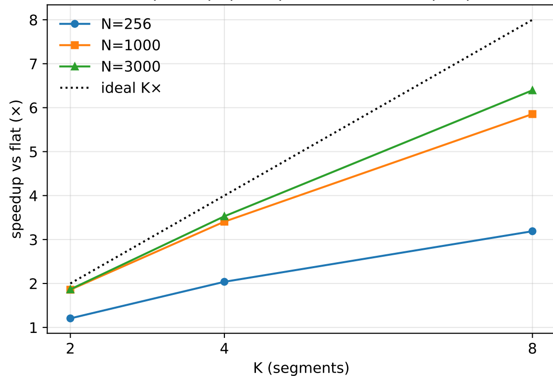
Parallel speedup, plain-product (isolated per-prover)
