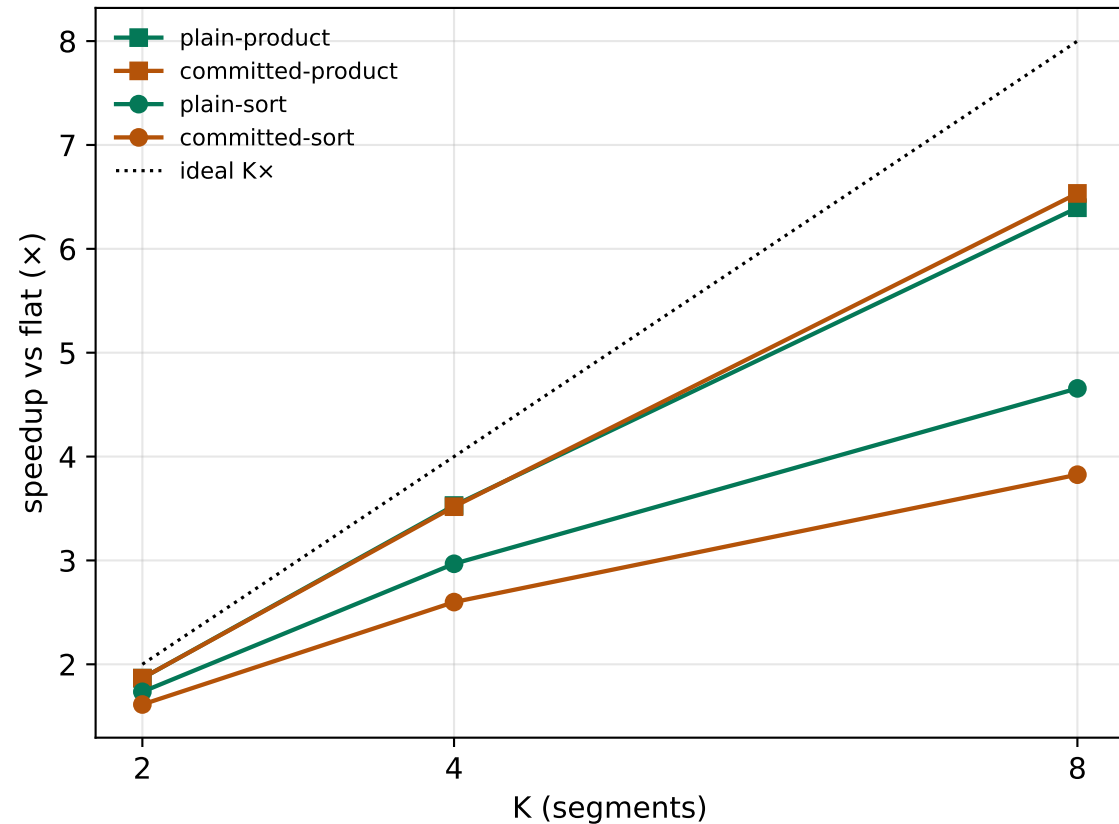
Parallel speedup (critical path = slowest segment + glue)
