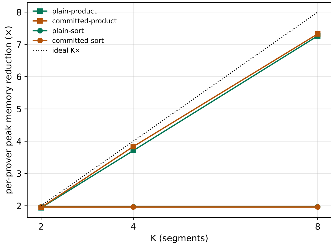
Per-prover peak memory reduction
