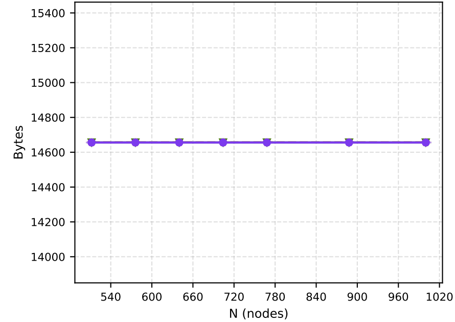
Proof size
