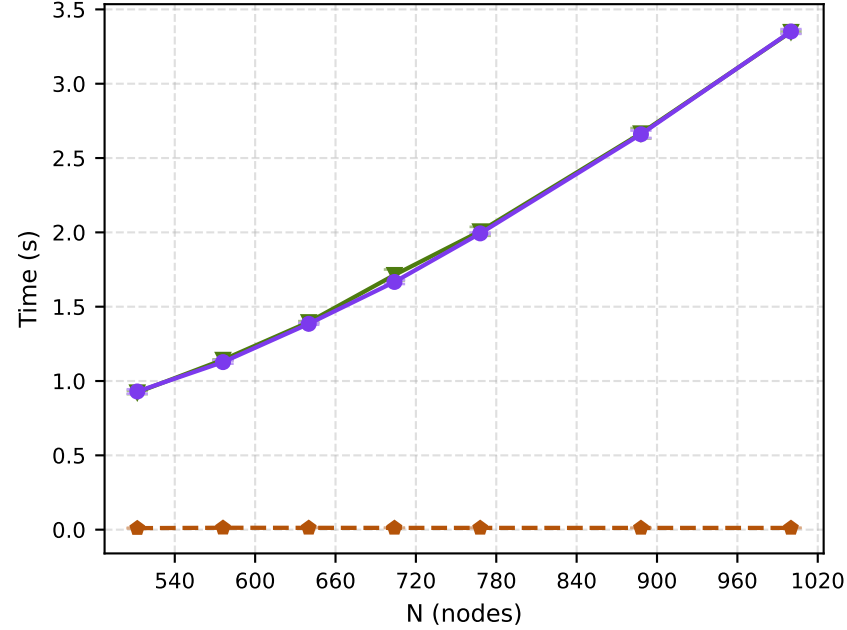
Compile time
