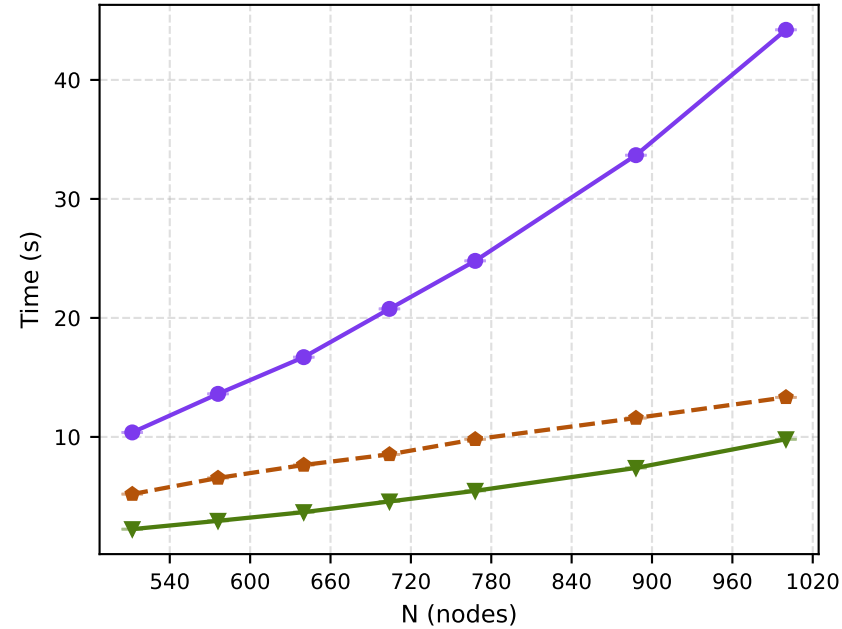
Compile time
