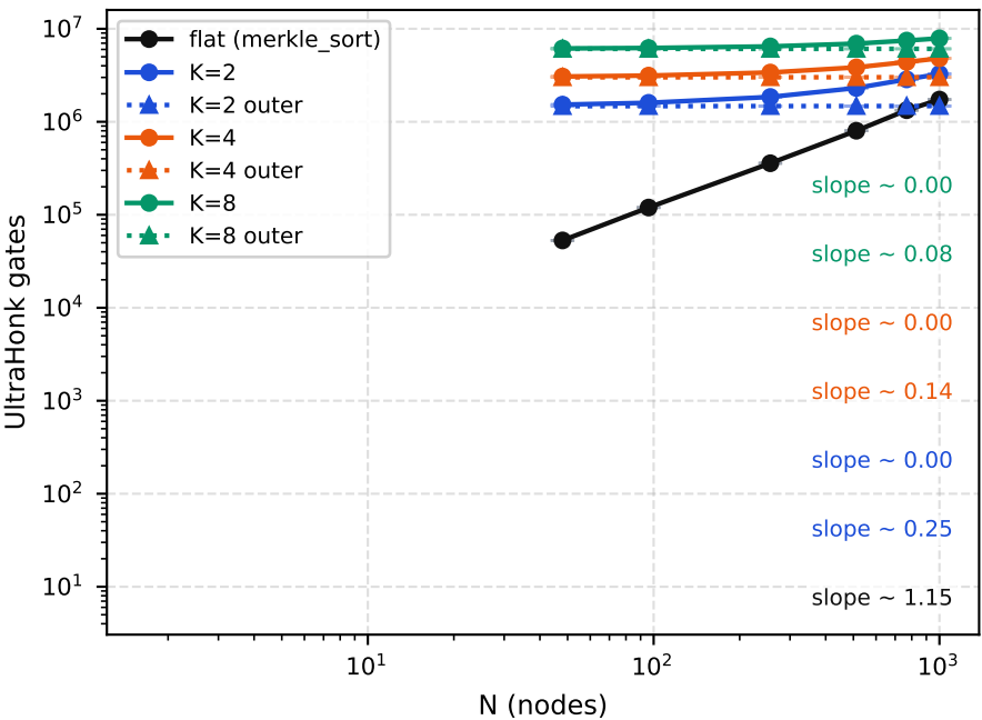
Circuit size (gates)
