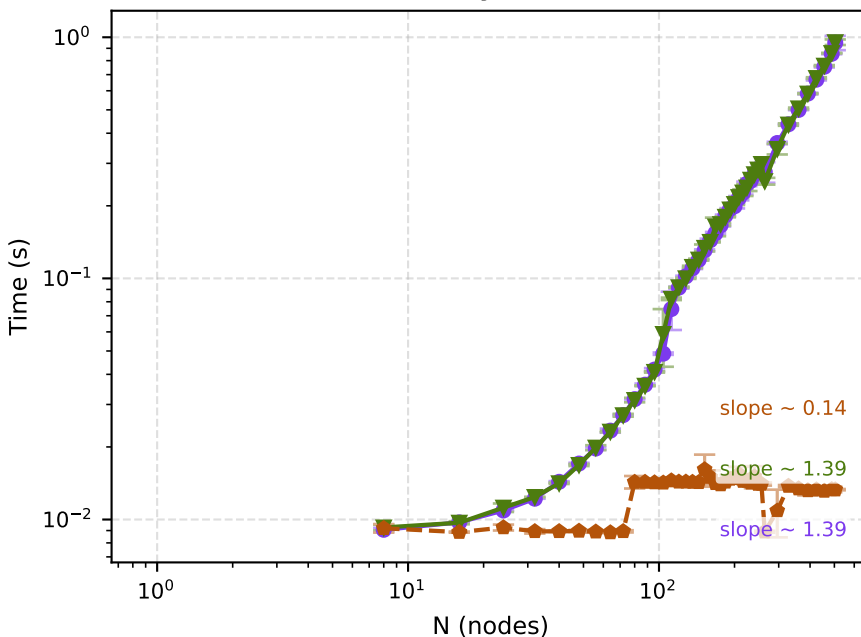
Compile time
