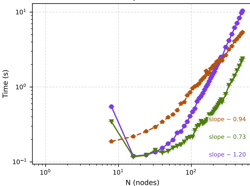
Compile time
