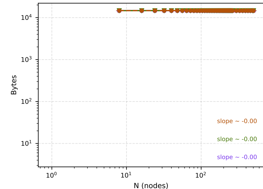
Proof size
