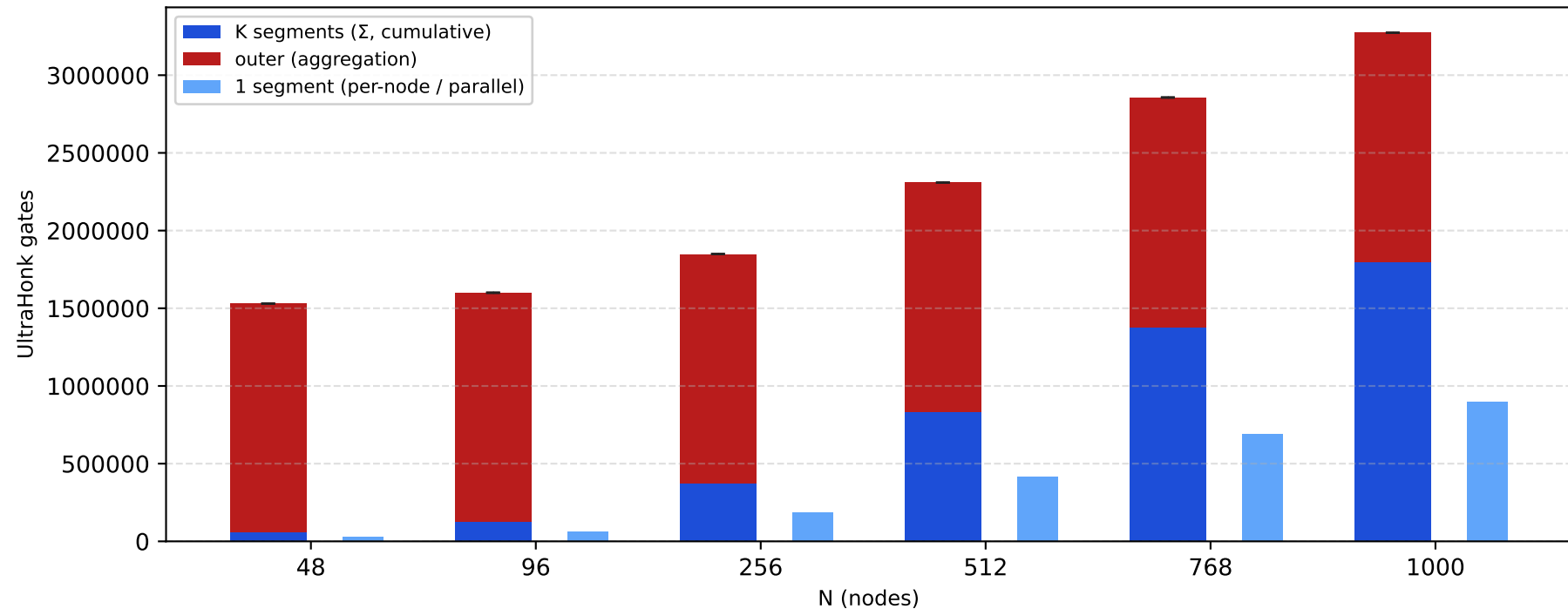
Circuit size (gates)
