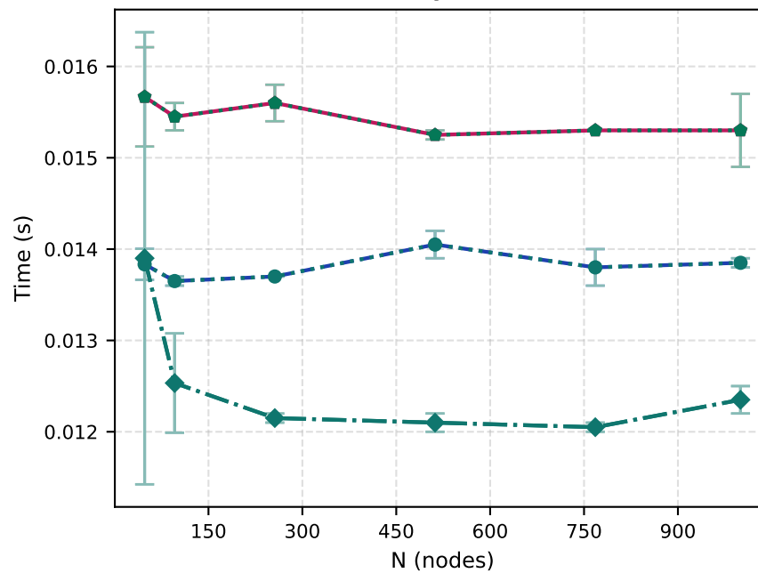
Compile time
