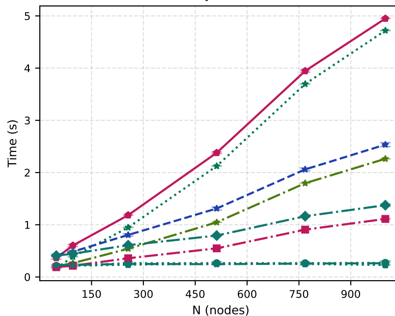
Compile time
