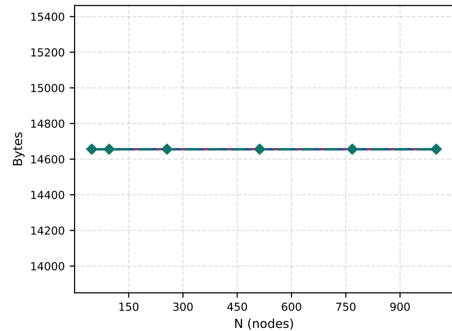
Proof size
