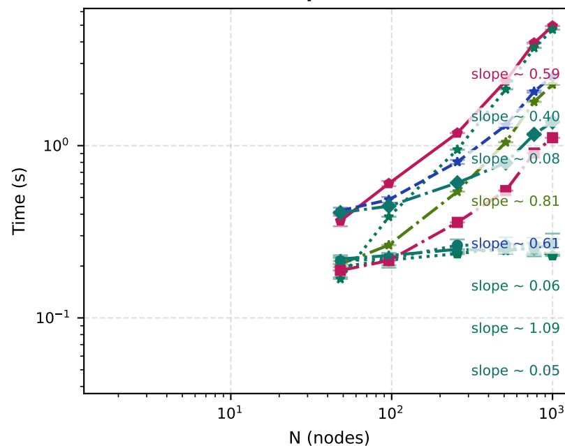
Compile time
