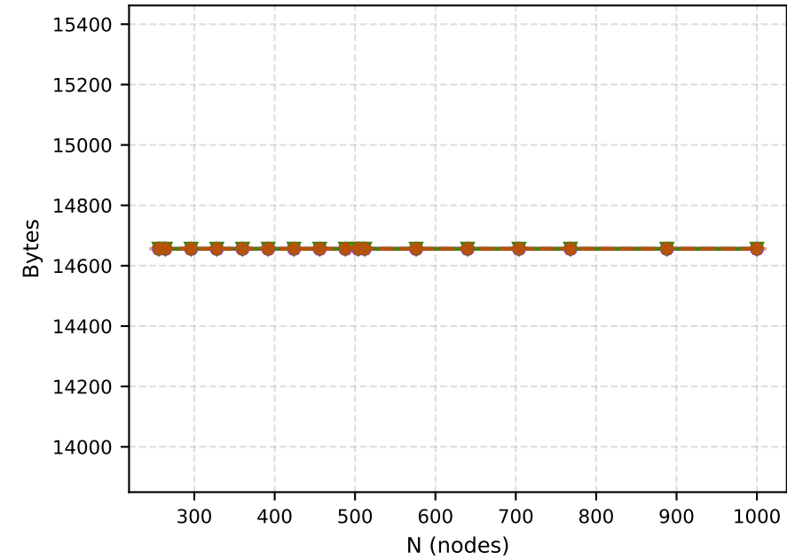
Proof size
