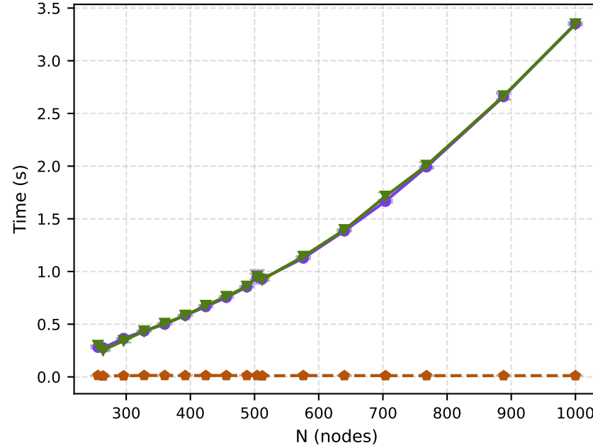
Compile time
