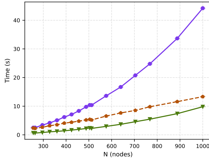
Compile time
