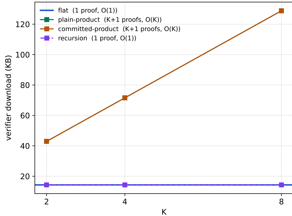
Proof bytes the verifier must check (n=1000)
