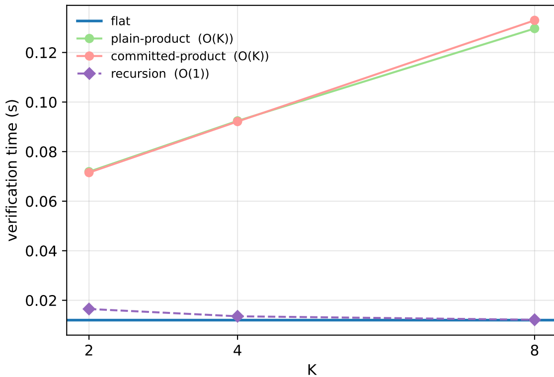
Verifier wall-clock
