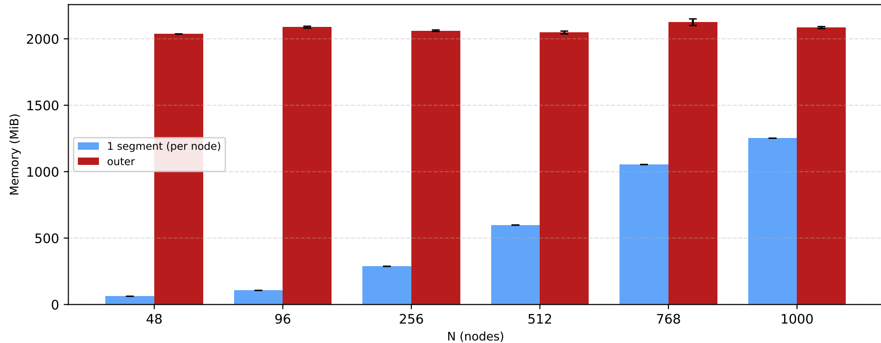
Peak memory (prove)
