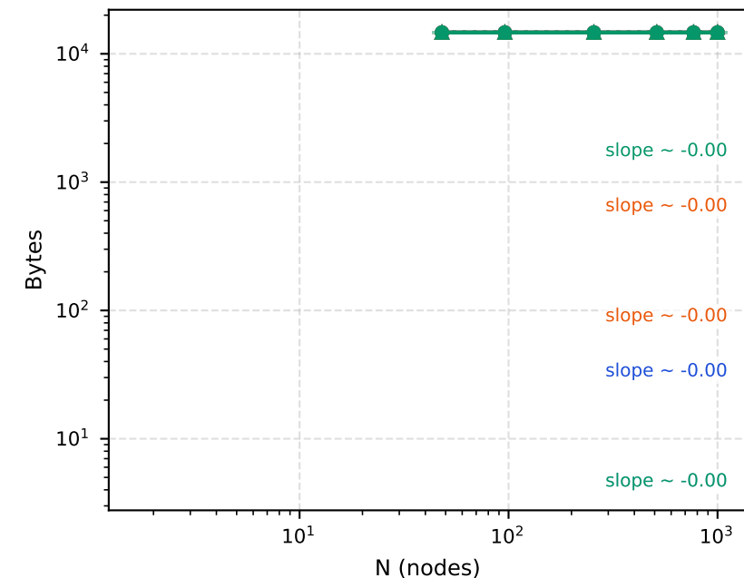
Proof size
