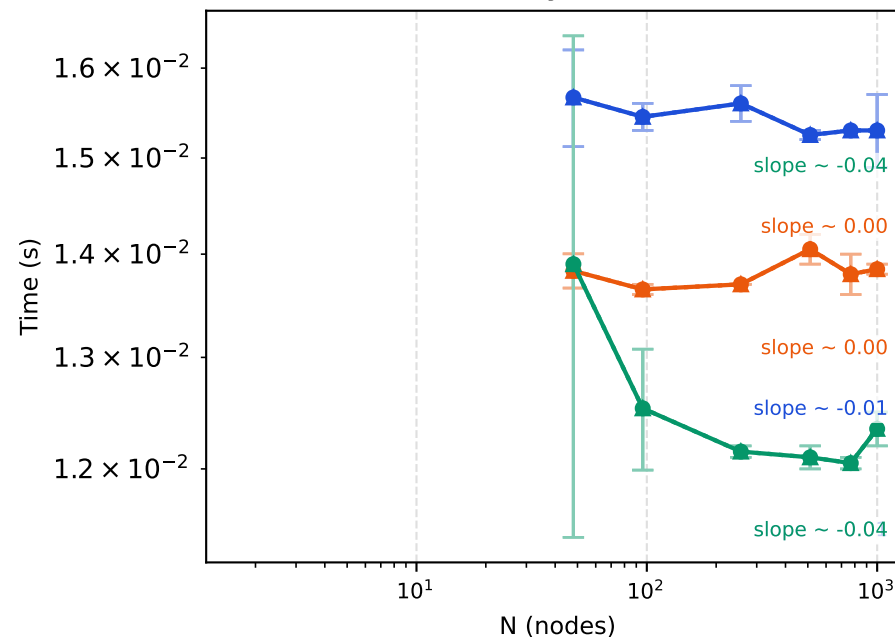
Compile time
