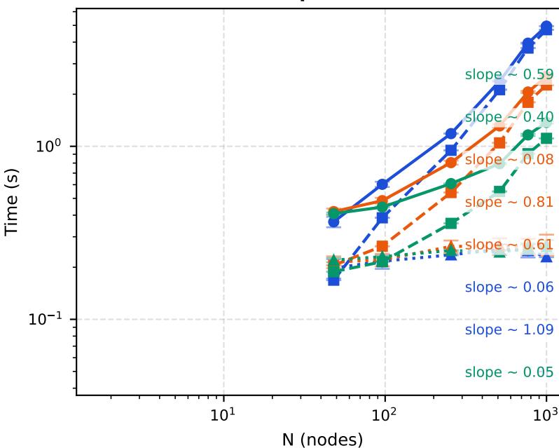
Compile time
