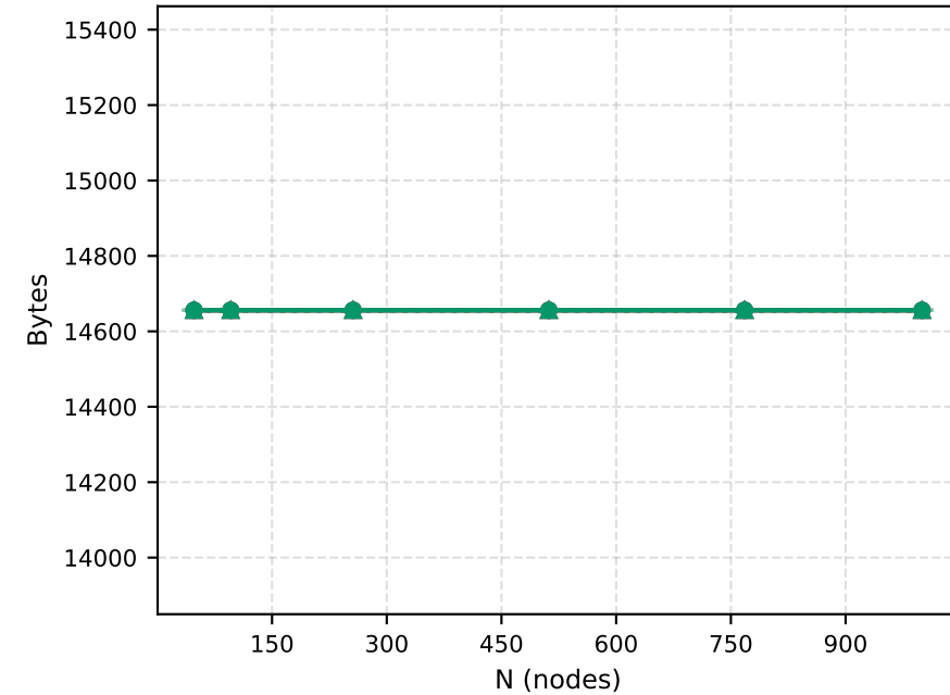
Proof size
