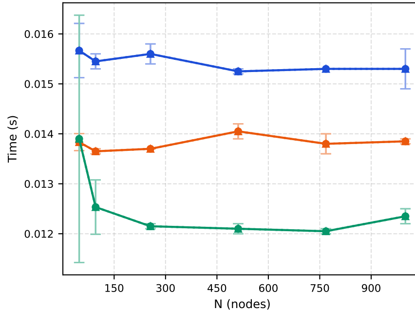
Compile time
