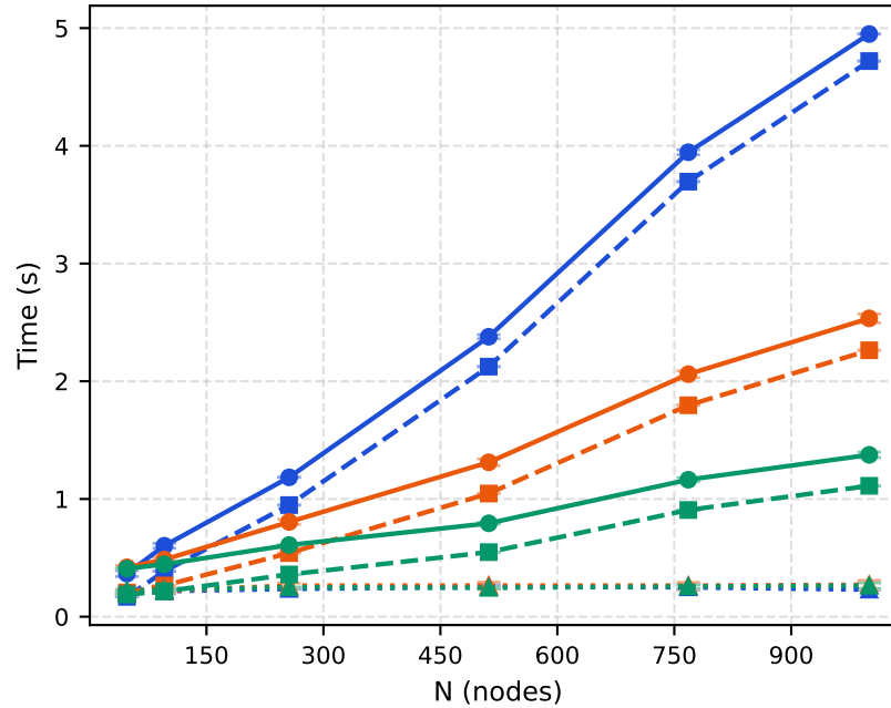
Compile time
