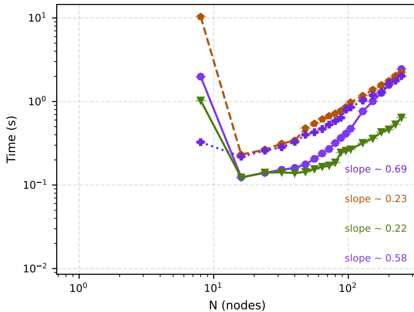
Compile time
