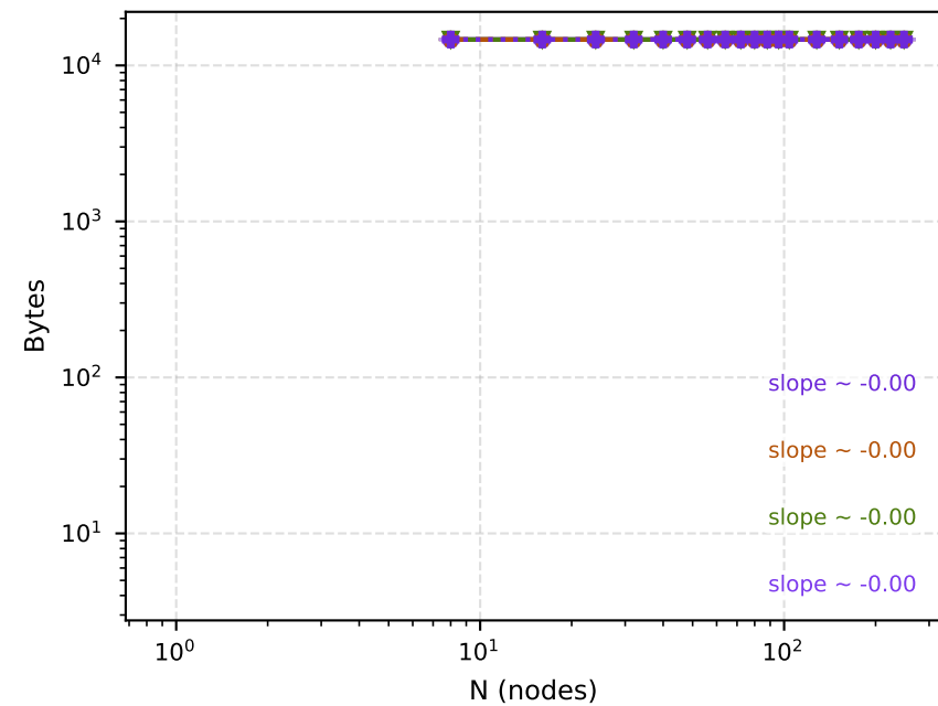
Proof size
