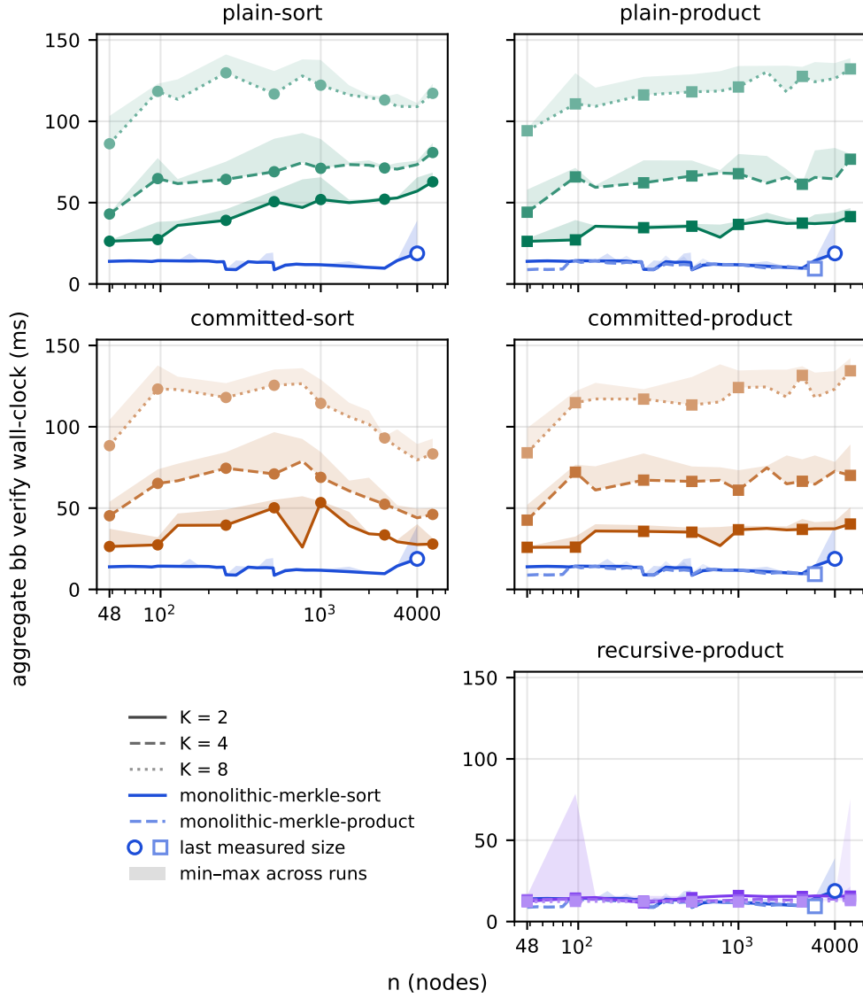
Figure 6.11: Aggregate bb verify wall-clock across the evaluation grid. External points sum the K + 1 required backend commands within each matched run; recursive points contain only the final outer verification. Curves show lower-envelope complete times and bands span the observed run-level minimum–maximum intervals. All panels use the same linear time scale and a logarithmic n -axis. Open markers identify the last measured reference points.
