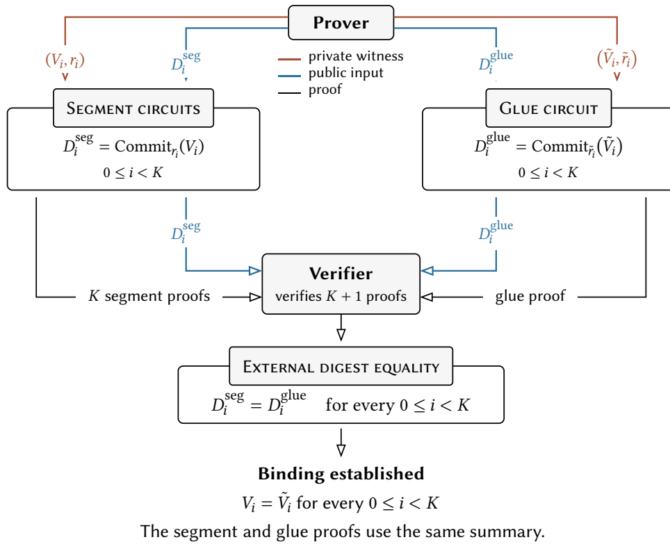
Figure 5.2: Committed specialization of Figure 5.1. Each circuit binds a private opening to its public digest copy, and the verifier requires the two copies to match.
