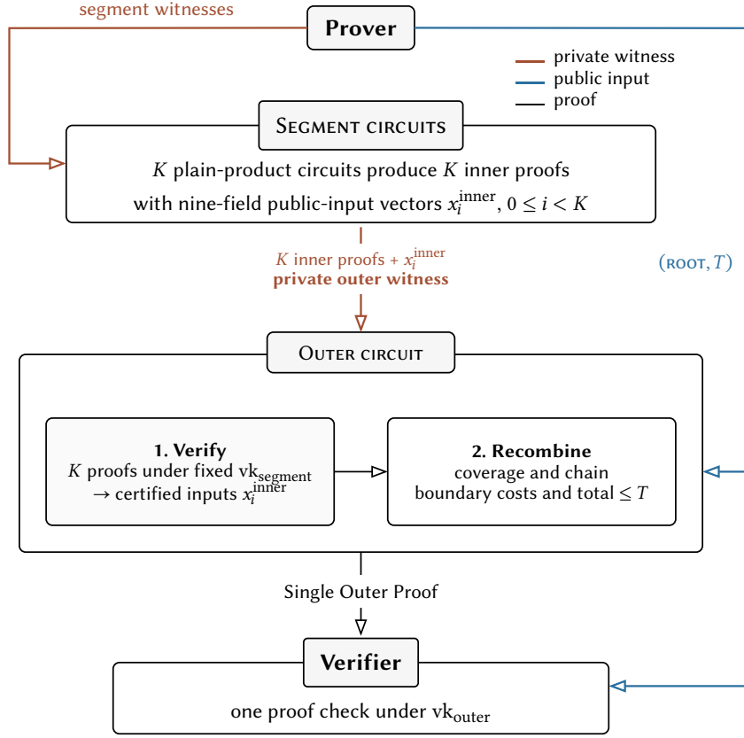
Figure 5.3: Recursive composition of the segment proofs. Each inner proof exposes a nine-field public-input vector x_i^{\text{inner}} at the inner-proof boundary; the proof and its vector together become private witness to the outer circuit. The outer circuit verifies the proofs under the fixed segment key, recombines their certified inputs, and emits a single outer proof with public interface (\text{ROOT}, T) .
