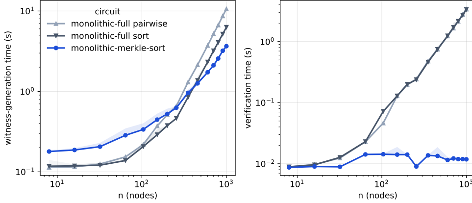
Figure 4.4: The two metrics not captured by gate count. Left: witness-generation time. Right: verification time. Times follow the lower-envelope convention of Figure 4.2.
