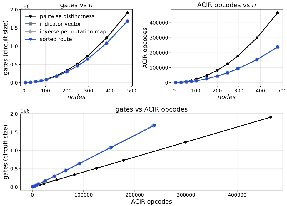
Figure 4.1: Three views of circuit size for different permutation mechanisms. Top left and top right show gate count and ACIR opcodes against the number of nodes, respectively. Bottom relates the two whole-circuit totals; it should not be interpreted as the gate price of an individual opcode.
