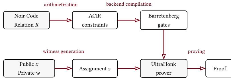
Figure 3.1: From relation to proof: static compilation and input-dependent witness generation join at the UltraHonk prover.
