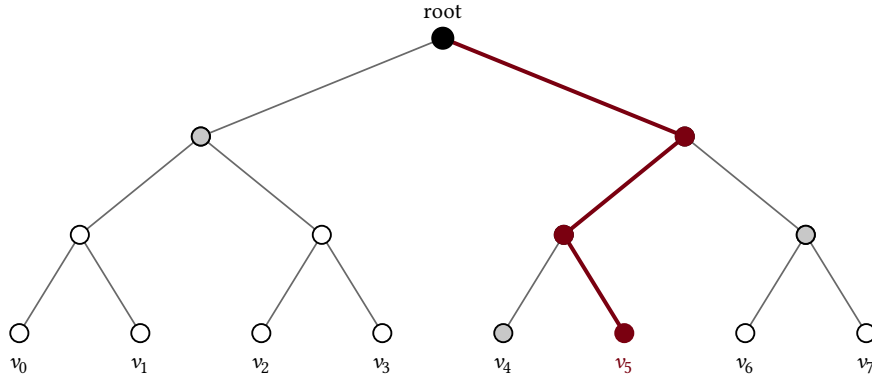
Figure 3.2: Authentication path for leaf v_5 in an eight-leaf Merkle tree. The dark path is recomputed from the opened leaf; the gray nodes are the three sibling hashes supplied with the opening. Their left or right positions bind the opening to index 5.
