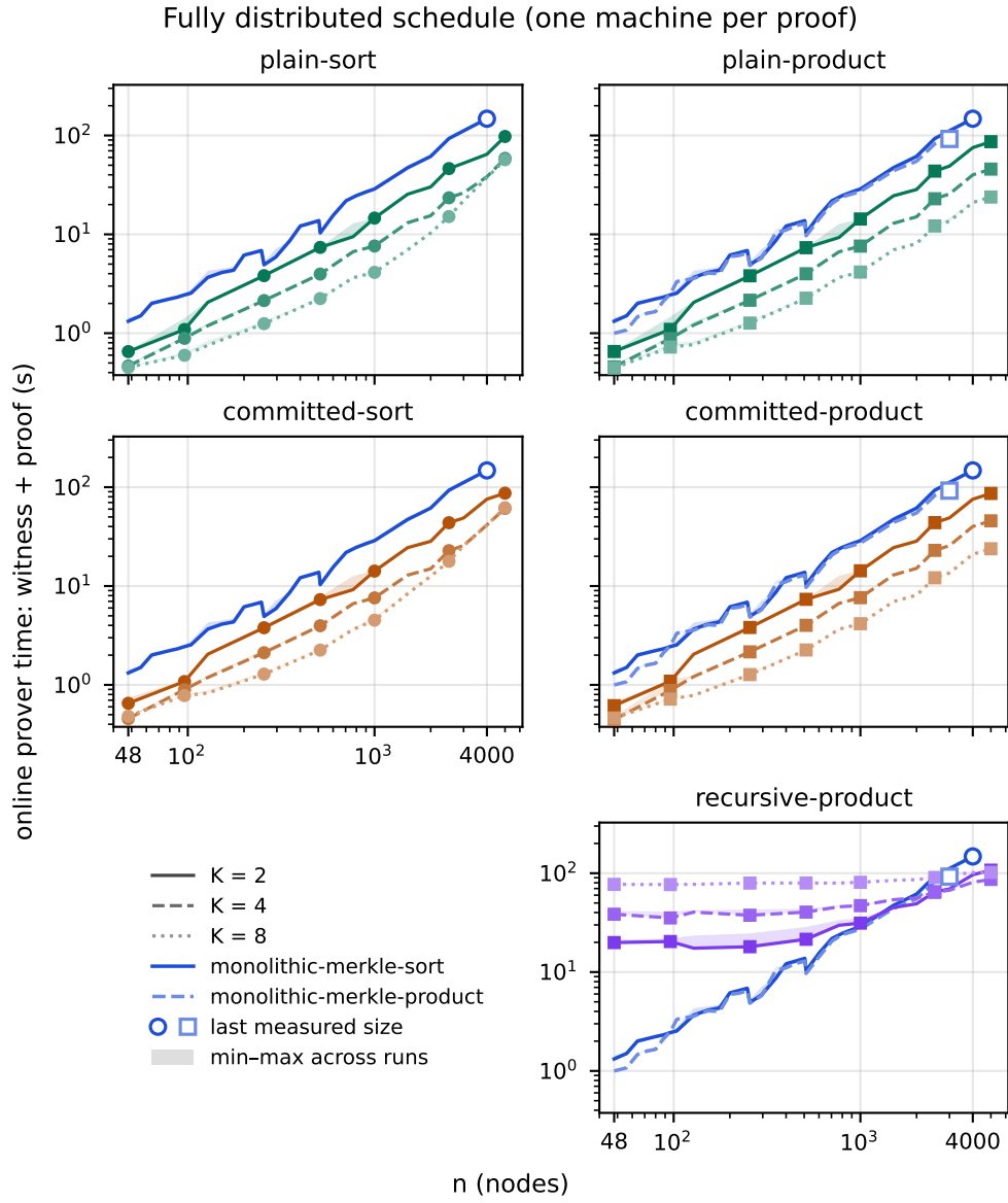
Figure 6.9: Fully distributed online prover-time estimates composed from the uncontended component runs. External completion is the maximum of the longest segment task and the independent glue task; recursive completion is the longest inner task followed by the dependent outer task. Curves show the lower-envelope run-level completion time and bands span the observed minimum–maximum range. The logarithmic axes are identical to Figure 6.8. The monolithic curves are single-host references: comparison with them is not hardware-normalized. The model assumes one comparable machine for each proof task that runs in parallel and excludes communication, coordination, and competition for shared host resources.
