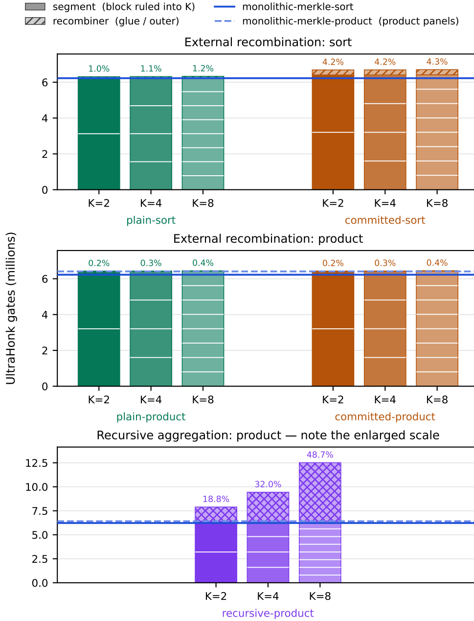
Figure 6.4: Distribution of aggregate UltraHonk gates at n = 3000 . Each bar contains K segment-circuit invocations and one recombination circuit. The unhatched block is the aggregate segment work and is divided into K equal slabs, each corresponding to one segment circuit; the hatched cap is the glue or recursive outer circuit. Percentages report the recombiner's share of the complete bar. Solid horizontal lines show monolithic Merkle-sort, while dashed lines in the product panels show monolithic Merkle-product. The external panels share a vertical scale; the recursive panel uses an enlarged scale.
