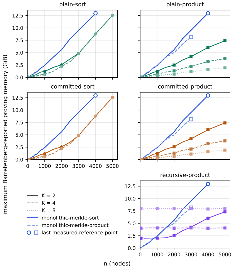
Figure 6.6: Median end-to-end maximum Barretenberg-reported proving memory for the five composite constructions. Within each matched run, the complete peak is the maximum over the K segment invocations and the glue or outer invocation. All panels use the same linear axes. The solid reference is monolithic Merkle-sort; product-based panels also show monolithic Merkle-product as a faint dashed control. Open markers identify the last measured reference points. Lines join measured checkpoints and are not extrapolated.
