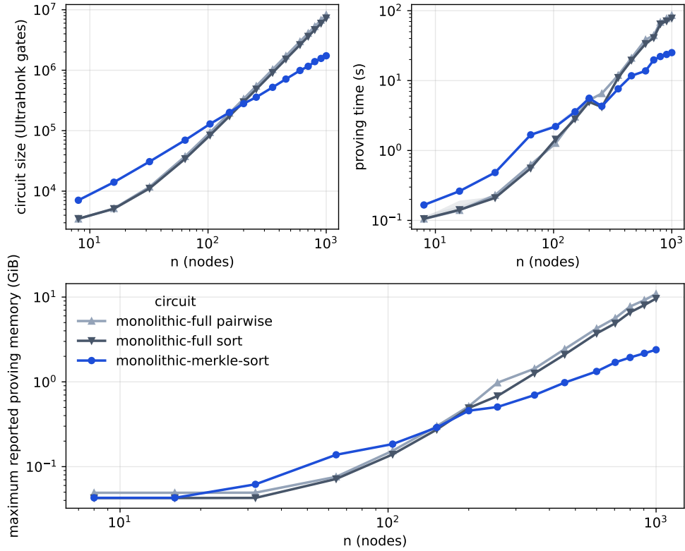
Figure 4.3: Circuit size, proving time, and maximum Barretenberg-reported proving memory through n = 1000 , on logarithmic axes. The full circuits retain the quadratic public-matrix surface; Merkle commitment replaces it with a constant-size interface. Timing curves show minima, memory curves show medians of the per-run maxima, and bands span the observed ranges, following Section 6.1.2.
