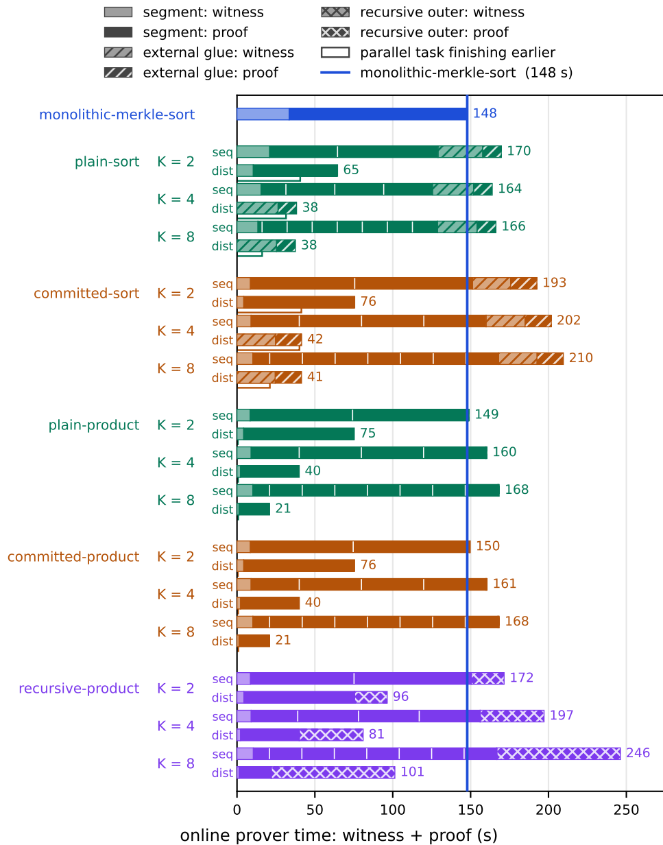
Figure 6.10: Sequential and fully distributed online prover-time composition for all constructions at n = 4000 . Filled distributed bars show the critical task or dependent task sequence; for external recombination, the unfilled outline is the parallel task that finishes earlier and is not added. Hatching distinguishes glue and the recursive outer stage. White rules divide aggregate segment witness-plus-proof time into K equal normalization shares rather than measured invocation boundaries. The blue bar and vertical rule mark the 147.8-second monolithic Merkle-sort reference. Monolithic product is unavailable at this checkpoint.
