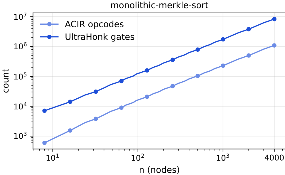
Figure 6.1: Compiler-level ACIR opcodes and backend UltraHonk gates for the refined monolithic circuit as the route length n increases. Both are deterministic counts for the fixed toolchain and are shown on logarithmic axes.
