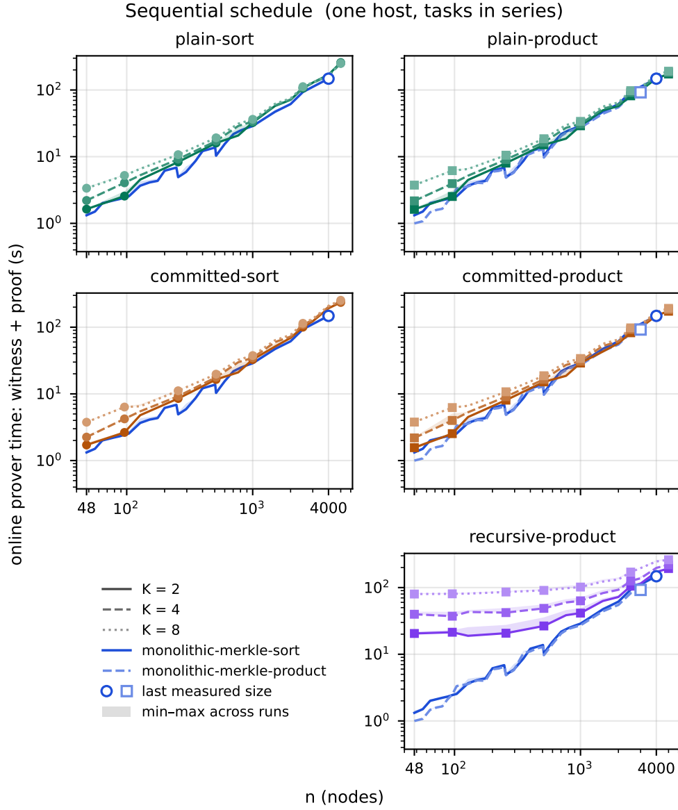
Figure 6.8: Sequential online prover time for the five composite constructions. Every point sums witness and proof generation over all K segment or inner invocations and the glue or outer invocation within a matched run. Curves show the lower-envelope complete time and bands span the observed run-level minimum–maximum range. Both axes are logarithmic and are shared with Figure 6.9. The solid reference is monolithic Merkle-sort; product-based panels also show monolithic Merkle-product as a faint dashed control. Open markers identify the last measured reference points. Lines join measured checkpoints and are not extrapolated.
