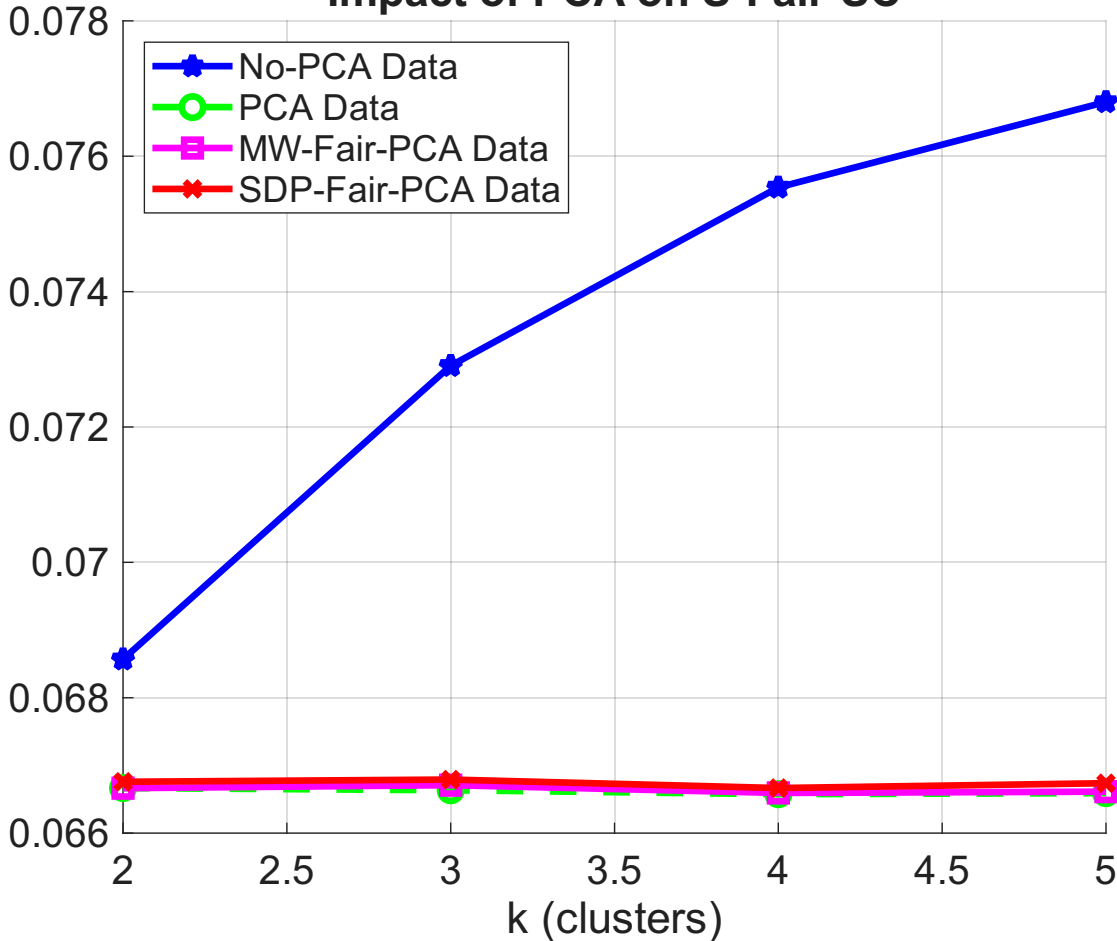
Impact of PCA on S-Fair-SC
