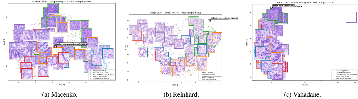
Figure 4.11 Shared UMAP (image embeddings + class-prompt markers, cosine metric) under each normalization. Compared to the baseline UMAP (Figure 4.3), Macenko shows clearly tighter benign-vs-malignant separation; Reinhard and Vahadane improve over baseline more modestly. Prompt markers still collapse in all three cases — every gain is image-side..
