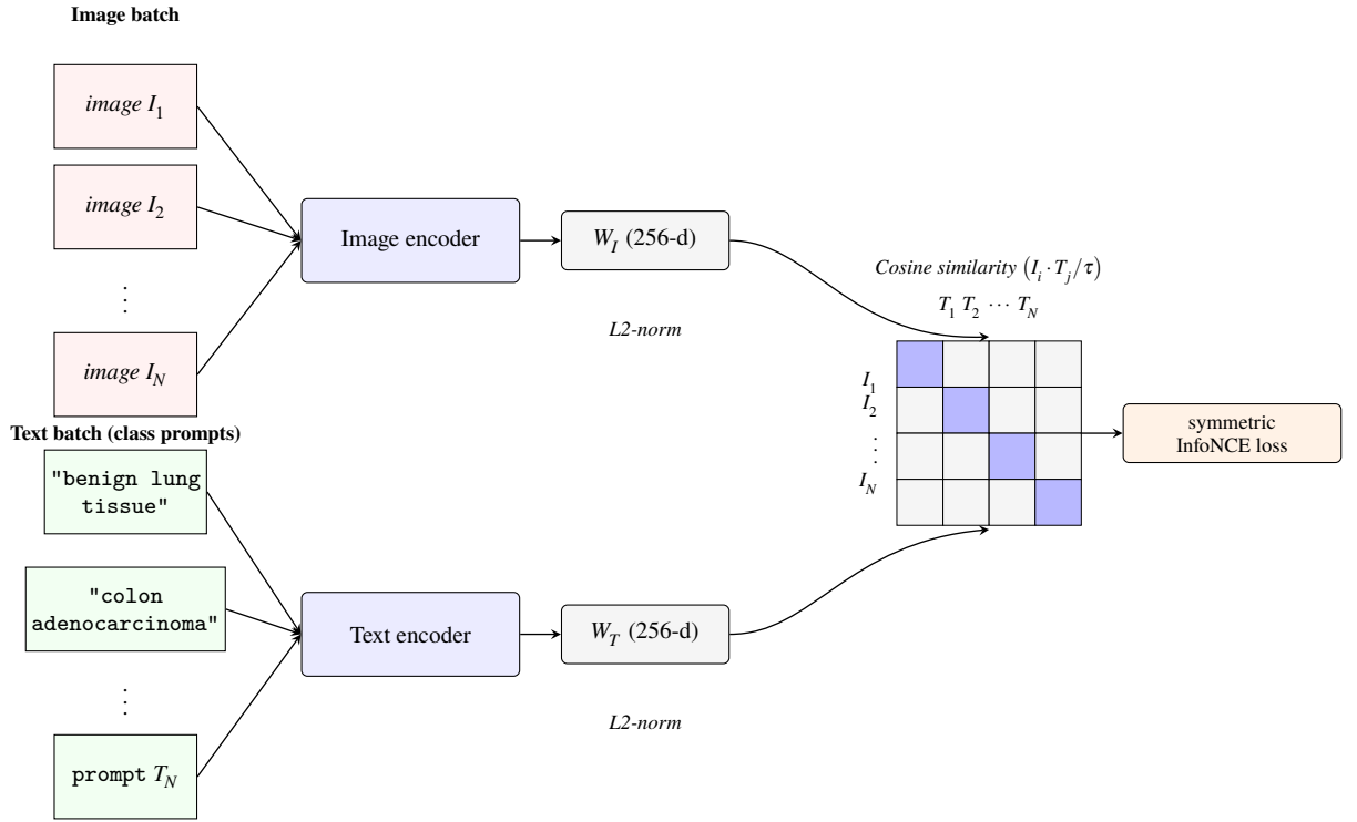
Figure 3.1 CLIP dual-encoder architecture used in this project. Two independent encoders project a batch of N image–text pairs into a shared d -dimensional embedding space (here d = 256 , the projection head’s output). After L2-normalisation and a learnable temperature \tau , the N \times N cosine-similarity matrix between every image and every prompt is the input to the symmetric InfoNCE loss. The diagonal (blue) entries are the positive pairs; off-diagonal entries are negatives within the batch..
