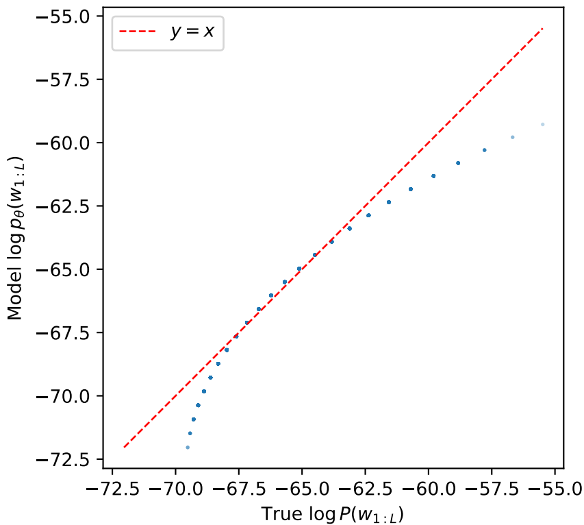
Best seed ( R^2=0.9737 )
