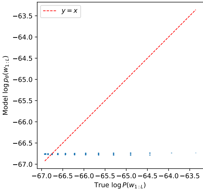
Best seed ( R^2=-0.0008 )
