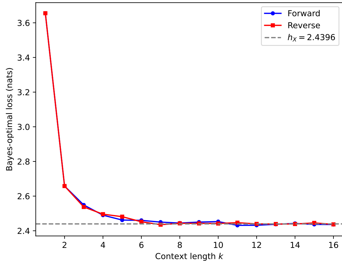
Bayes-optimal loss L^*(k)
