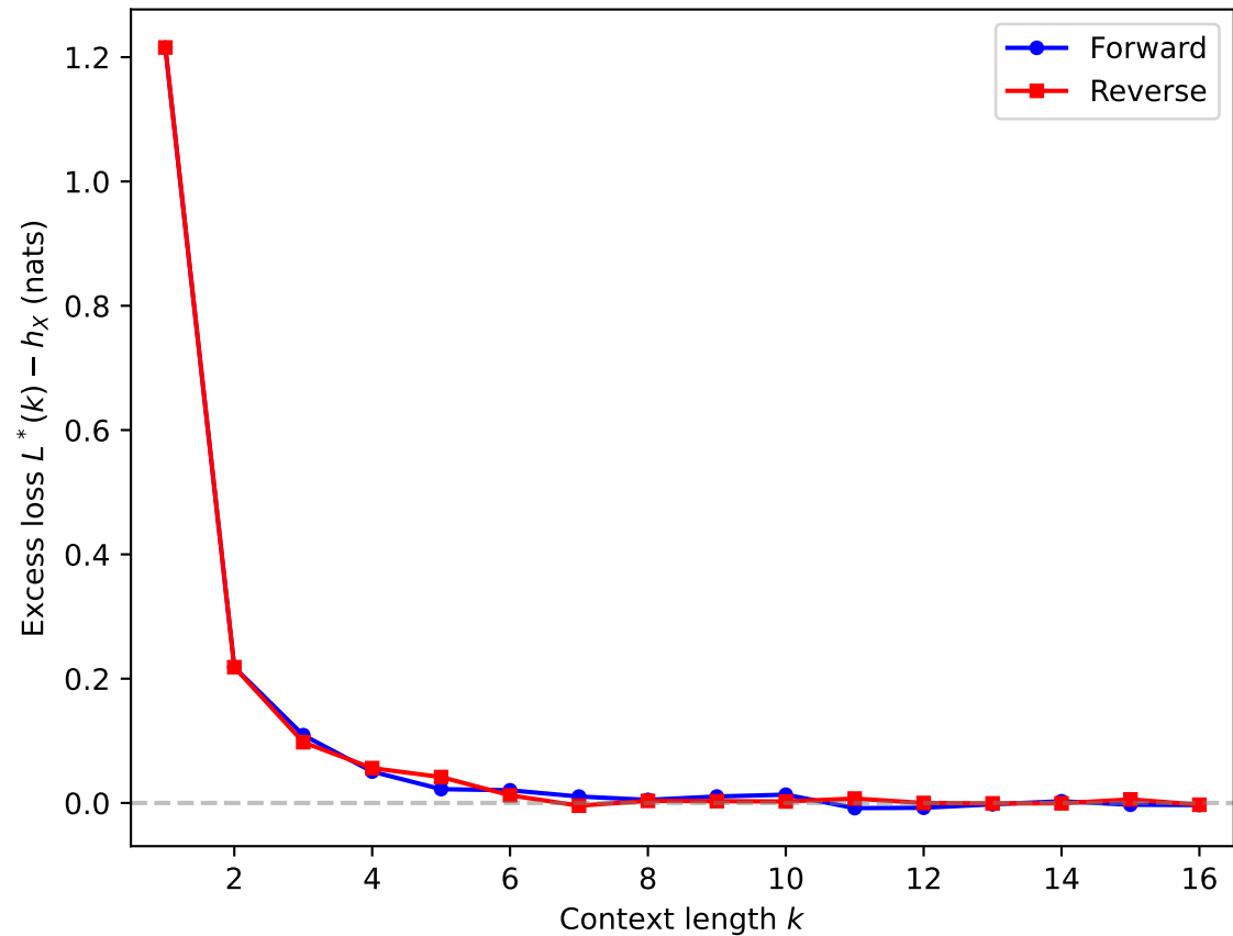
Excess Bayes-optimal loss
