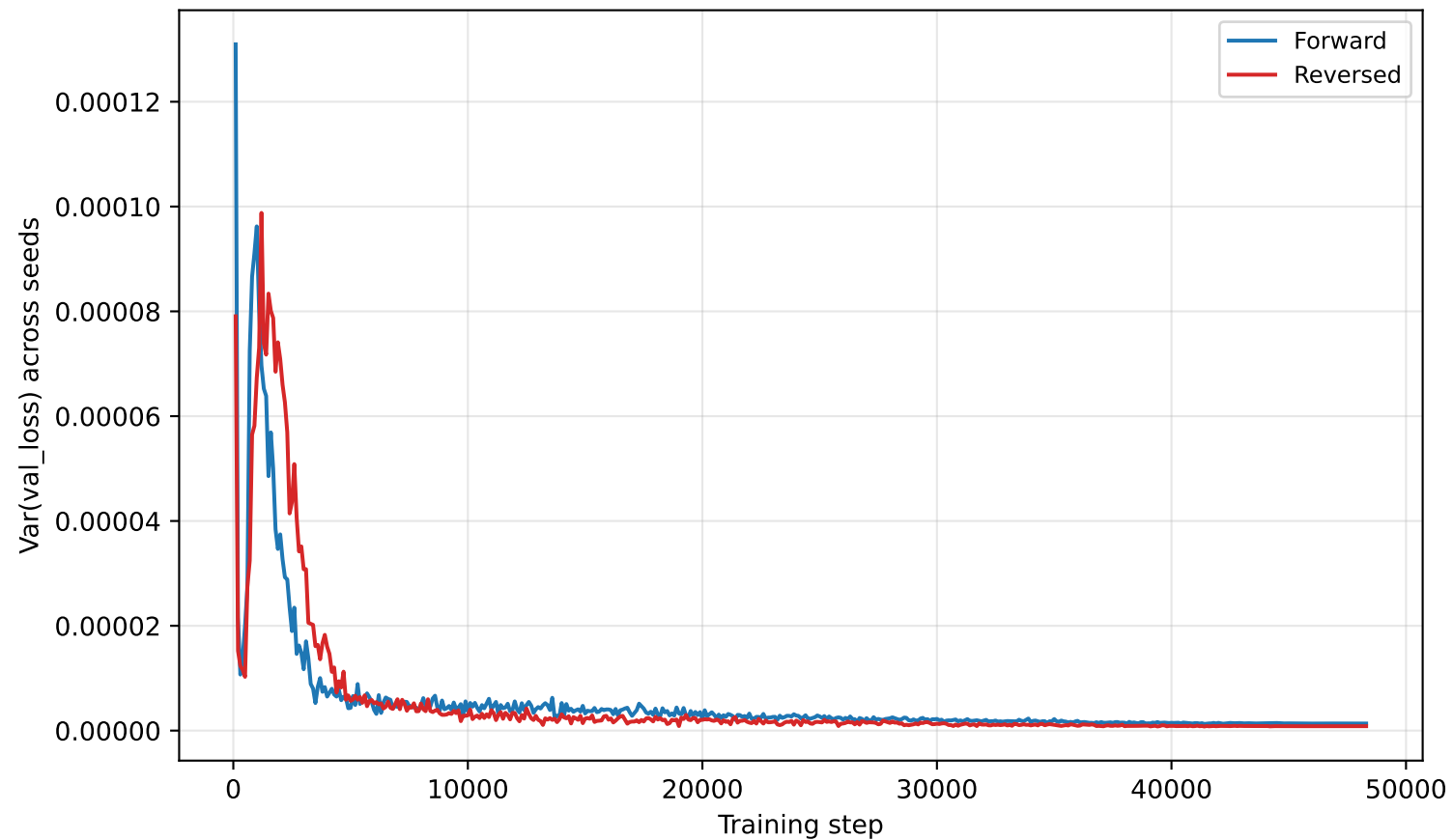
Loss variance evolution
