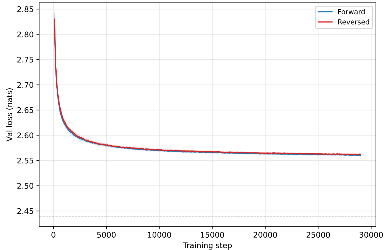
(b) Early training dynamics (first 20%)
