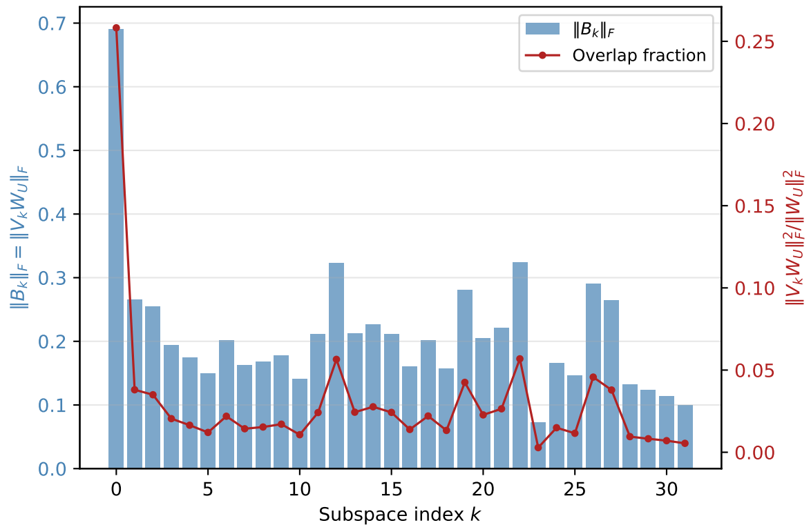
(B) W_U block scale per subspace
