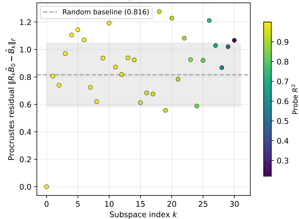
(A) Geometric alignment with subspace 0
